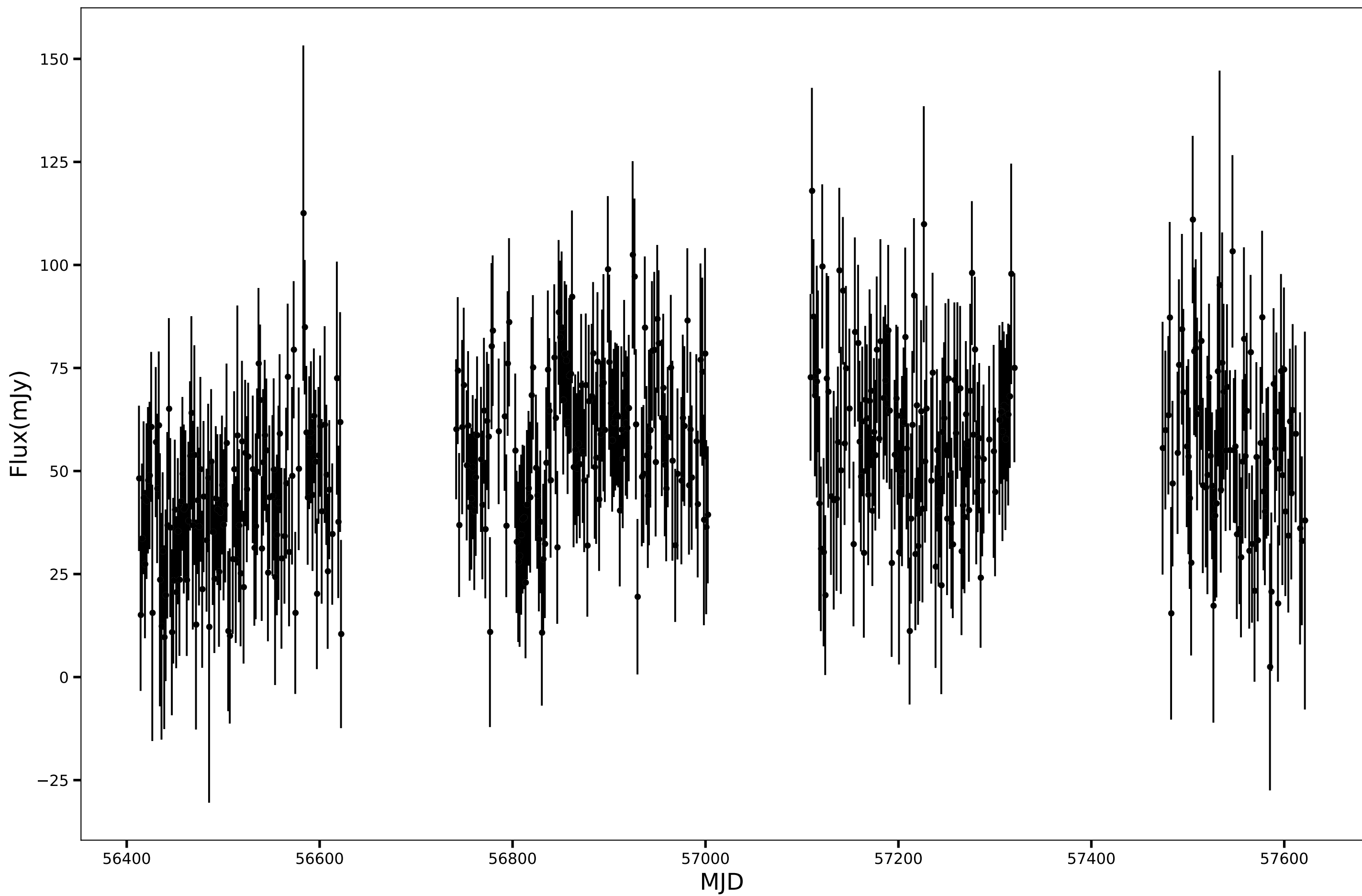
SPT-SJ224017-5232.0, RA=340.0744d, DEC=-52.5336d, mean_flux=53.39 (mJy), 90GHz
