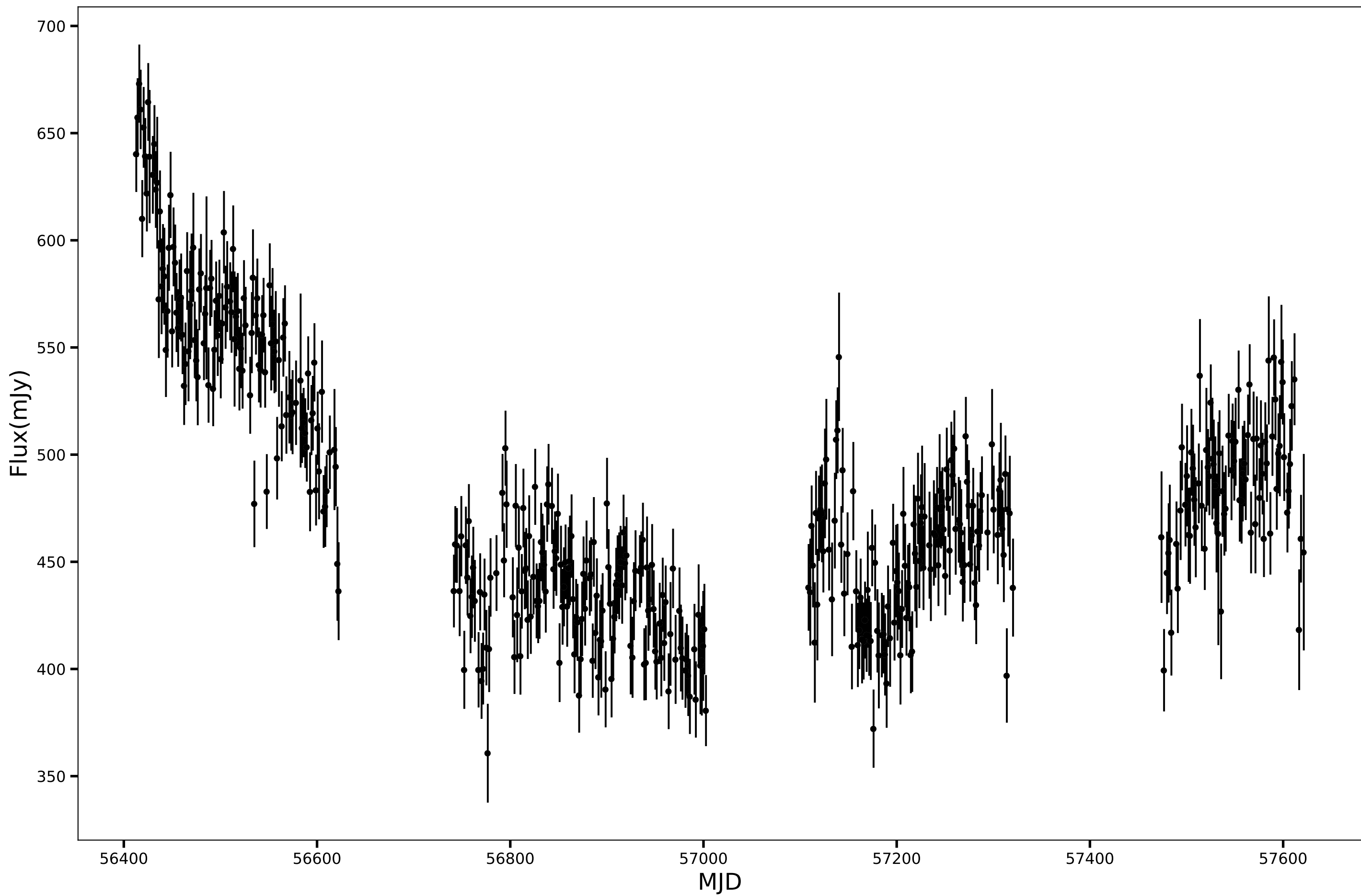
SPT-SJ223911-5701.0, RA=339.7999d, DEC=-57.0167d, mean_flux=479.87 (mJy), 90GHz
