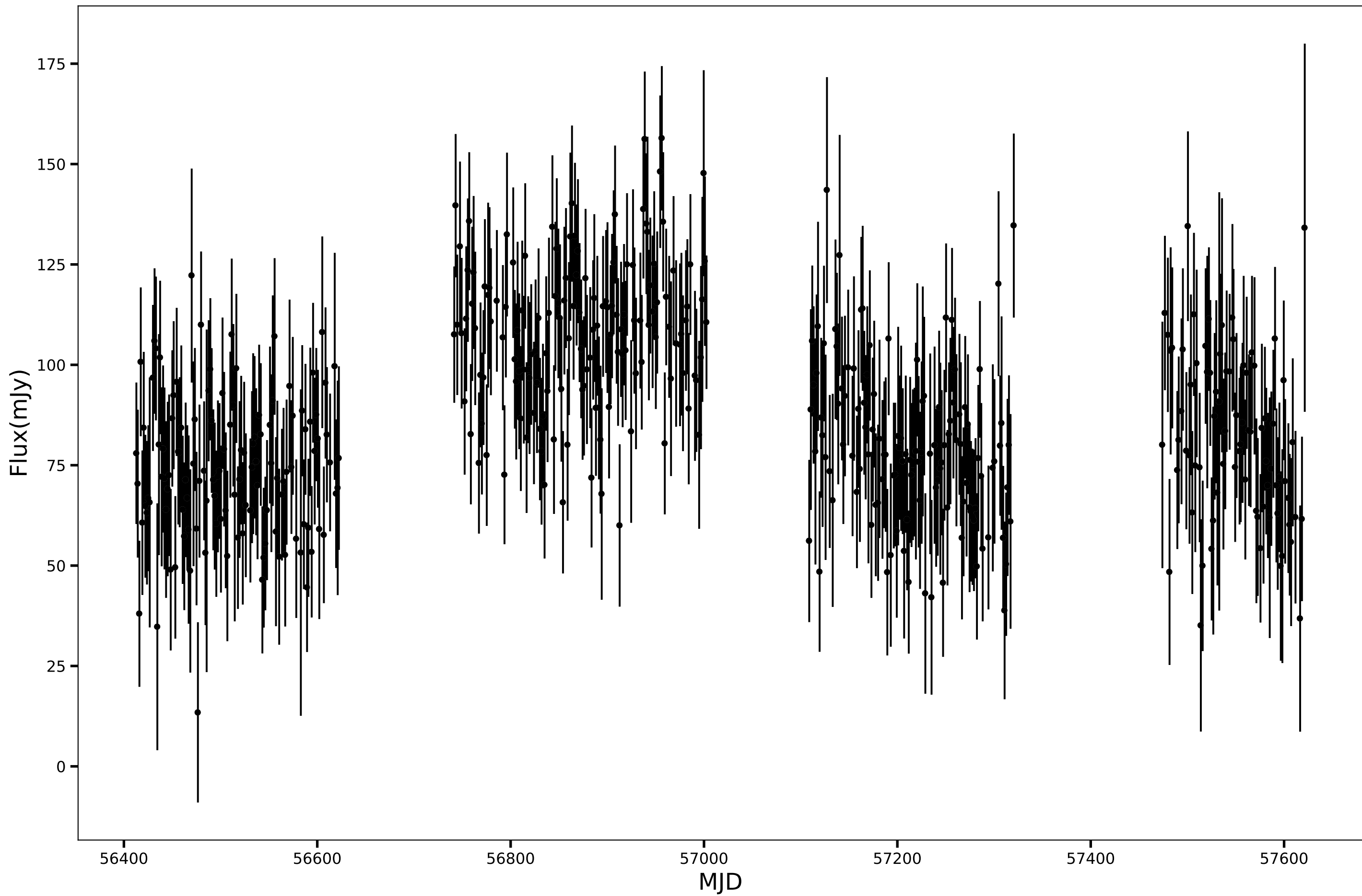
SPT-SJ223905-5526.0, RA=339.7745d, DEC=-55.4347d, mean_flux=87.38 (mJy), 90GHz
