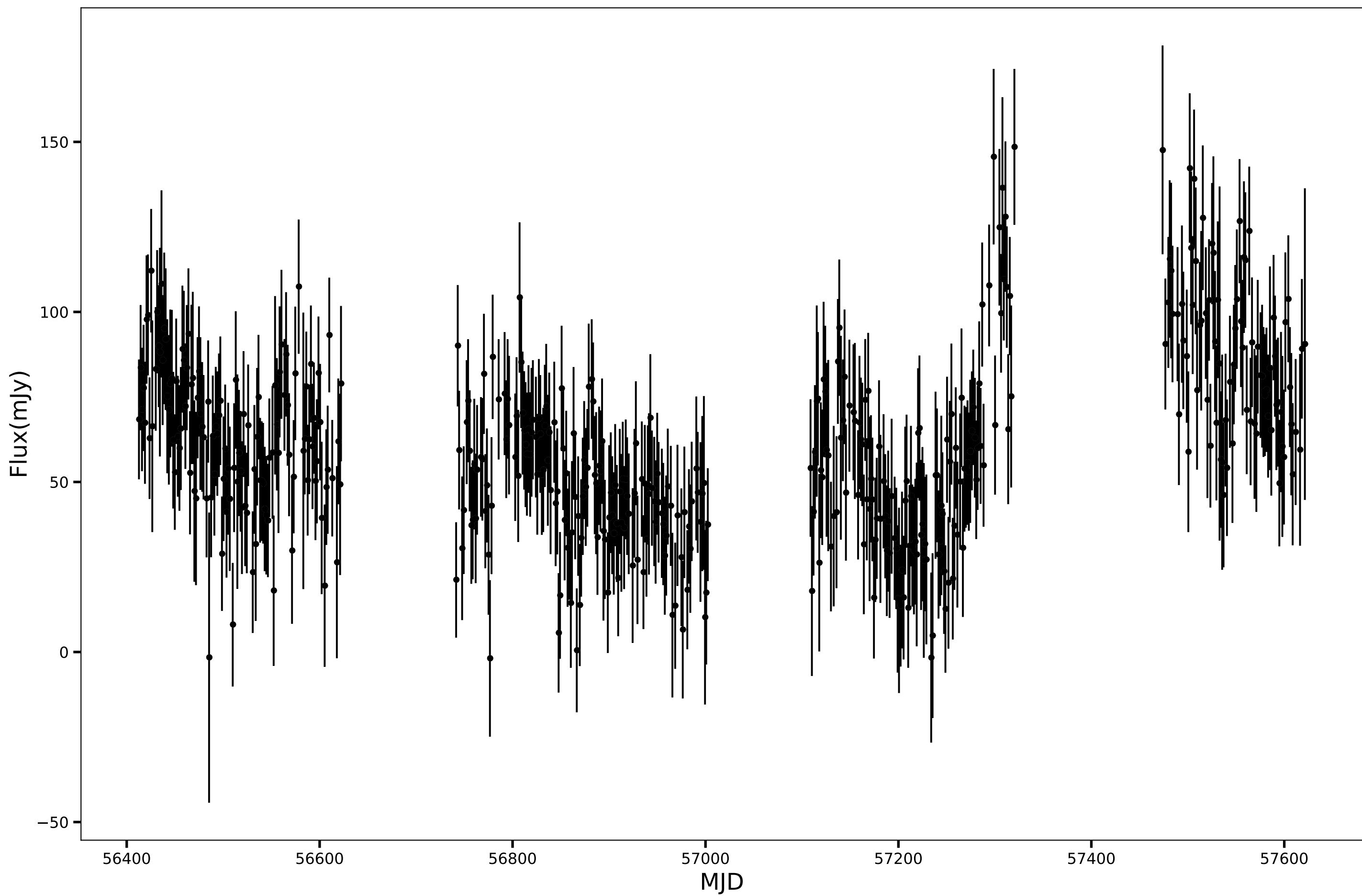
SPT-SJ223825-5114.3, RA=339.6050d, DEC=-51.2397d, mean_flux=60.37 (mJy), 90GHz
