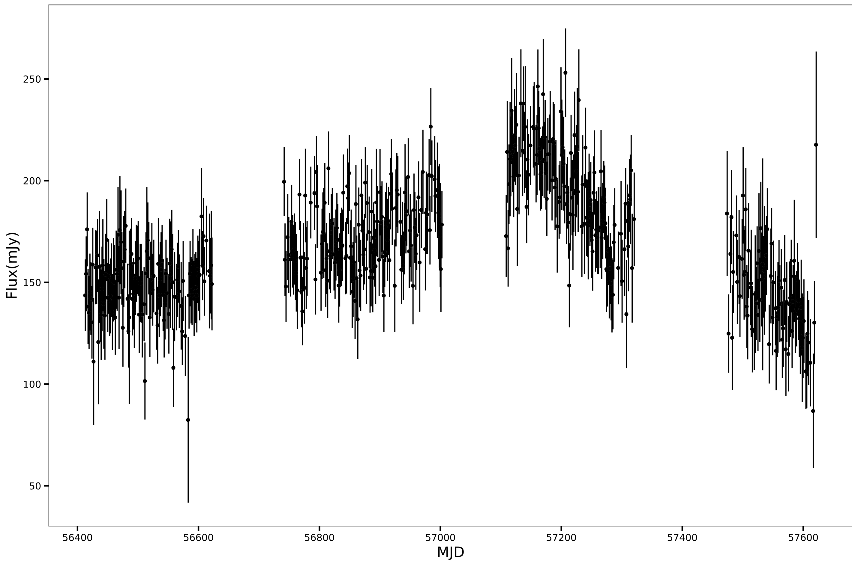
SPT-SJ223108-6231.3, RA=337.7861d, DEC=-62.5222d, mean_flux=167.20 (mJy), 90GHz
