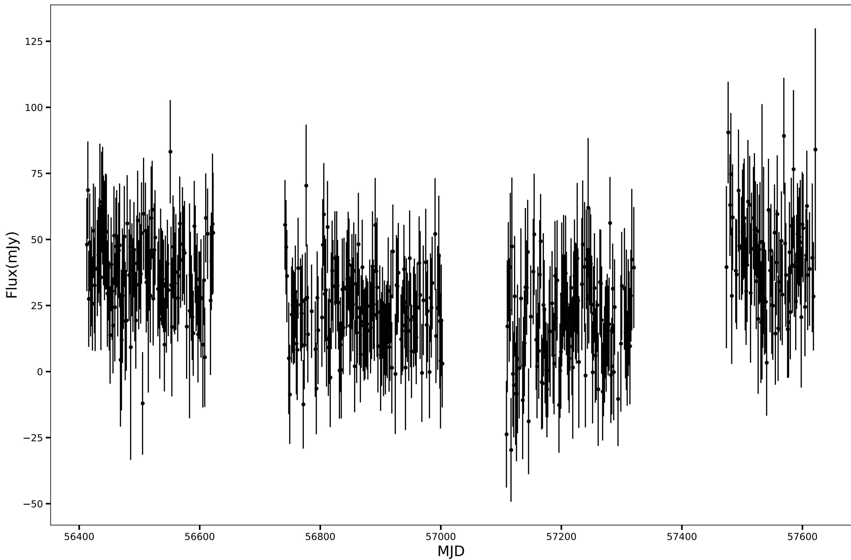
SPT-SJ223044-6329.4, RA=337.6842d, DEC=-63.4901d, mean_flux=29.13 (mJy), 90GHz
