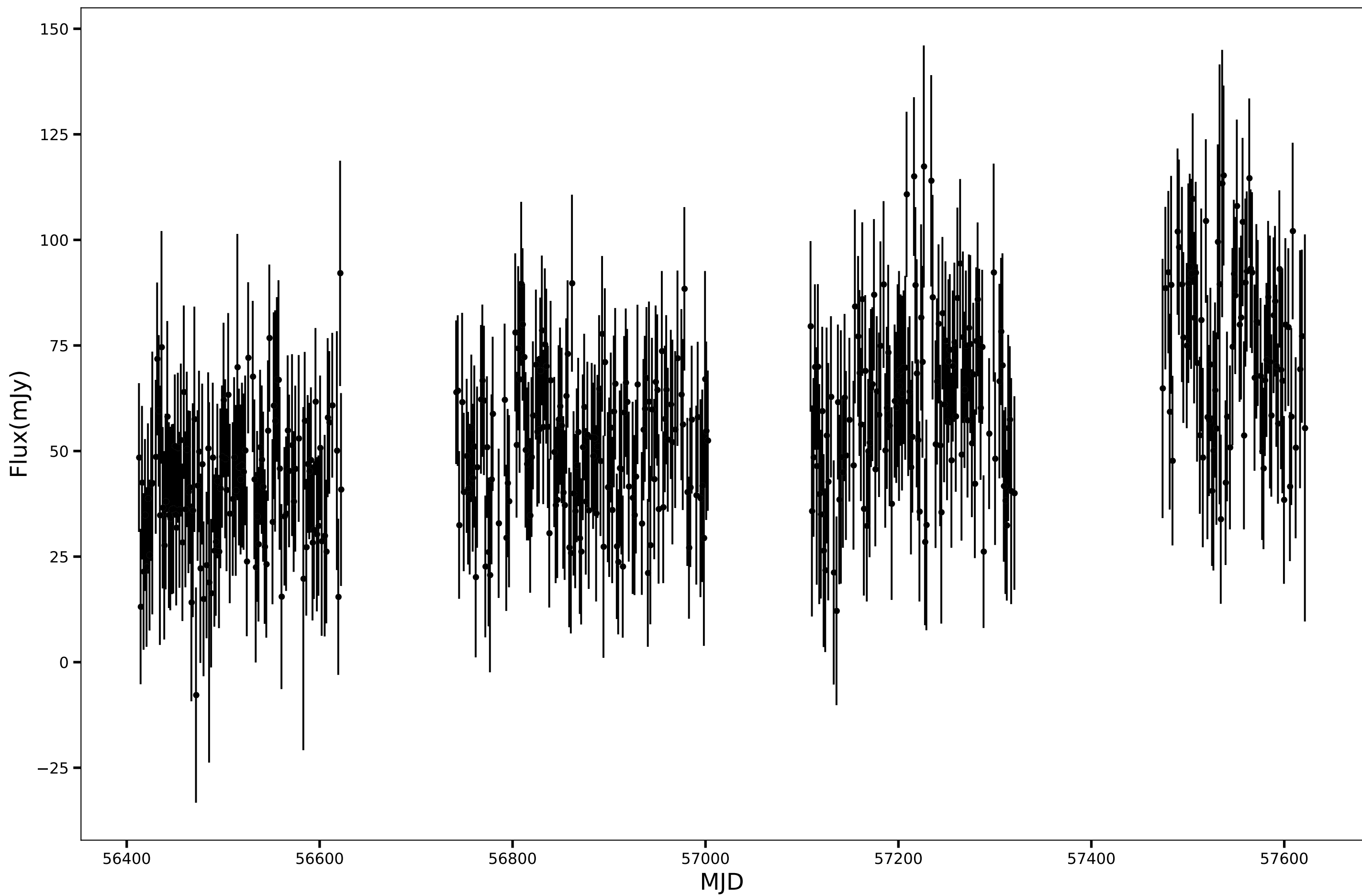
SPT-SJ222707-5219.9, RA=336.7831d, DEC=-52.3329d, mean_flux=55.45 (mJy), 90GHz
