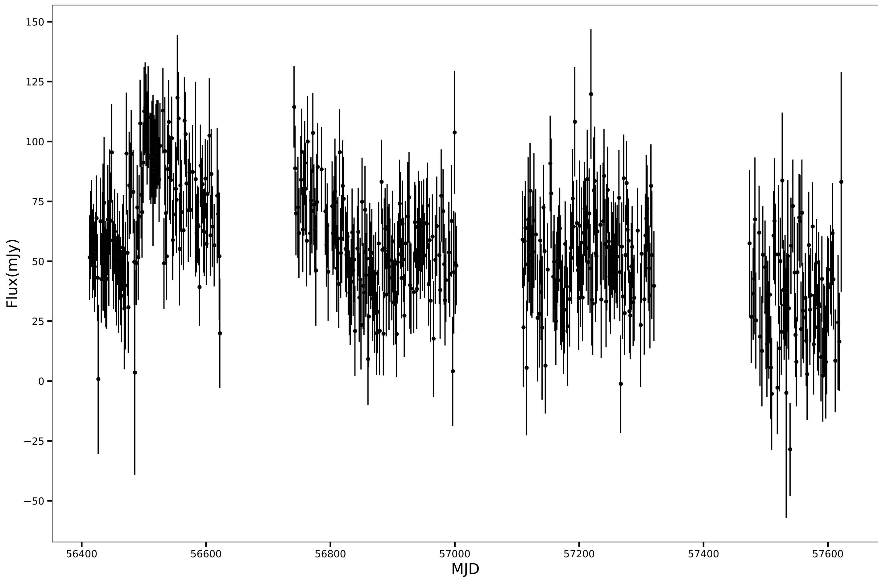
SPT-SJ221824-6454.6, RA=334.6038d, DEC=-64.9110d, mean_flux=55.16 (mJy), 90GHz
