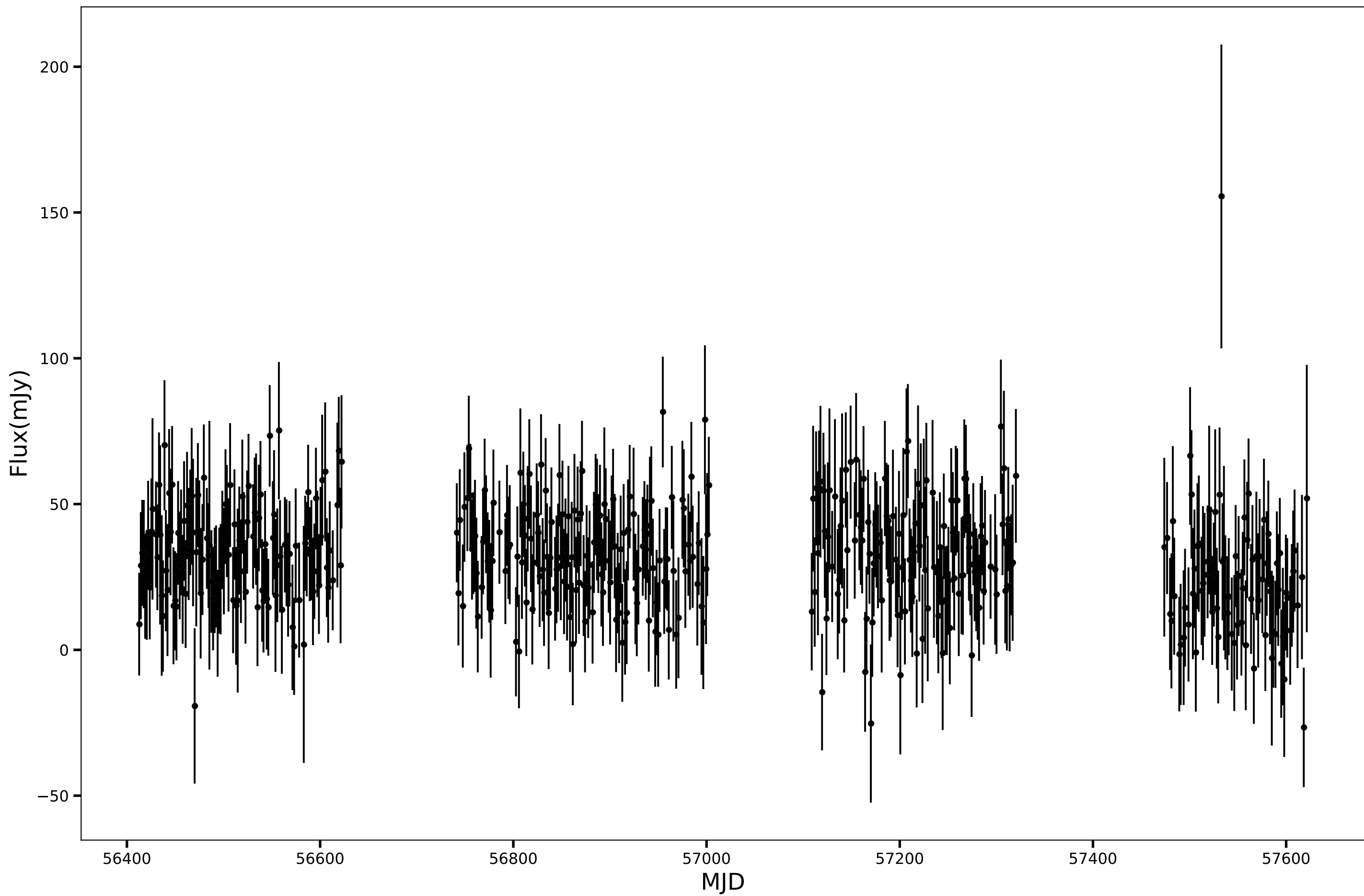
SPT-SJ221818-5038.6, RA=334.5765d, DEC=-50.6445d, mean_flux=31.67 (mJy), 90GHz
