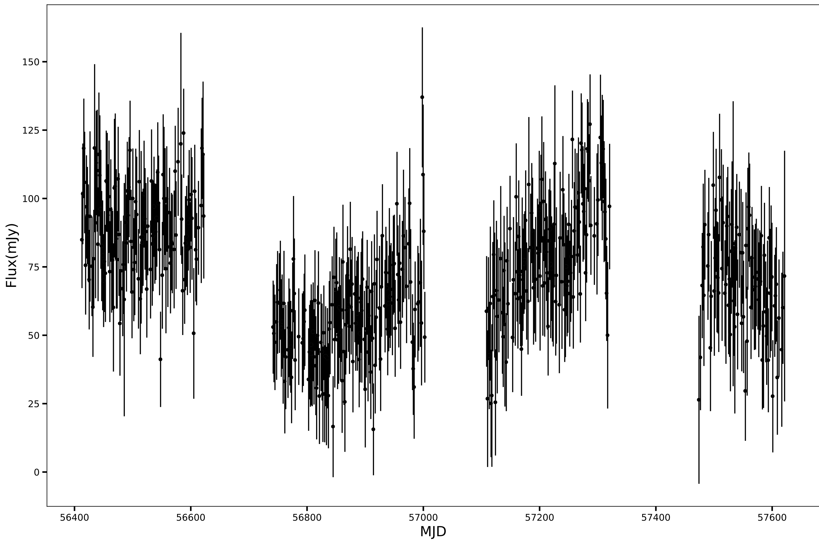
SPT-SJ221334-6329.9, RA=333.3919d, DEC=-63.4998d, mean_flux=72.95 (mJy), 90GHz
