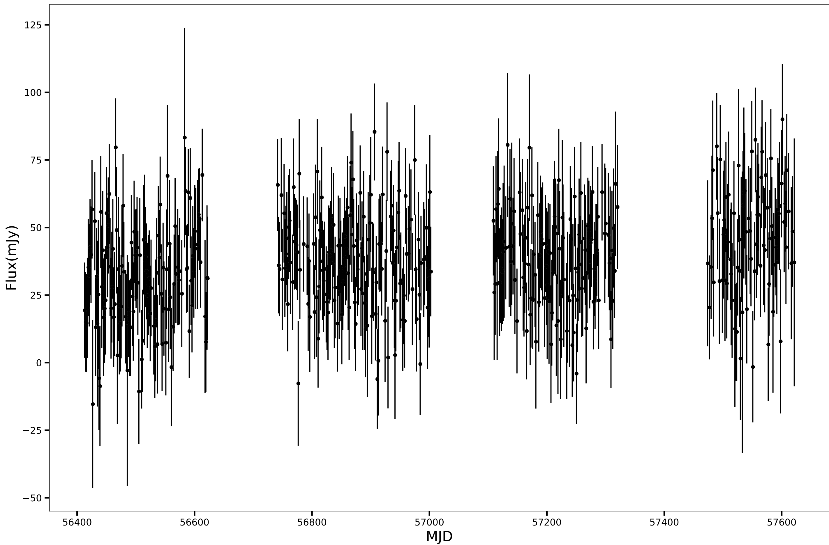
SPT-SJ221032-5508.6, RA=332.6343d, DEC=-55.1437d, mean_flux=37.42 (mJy), 90GHz
