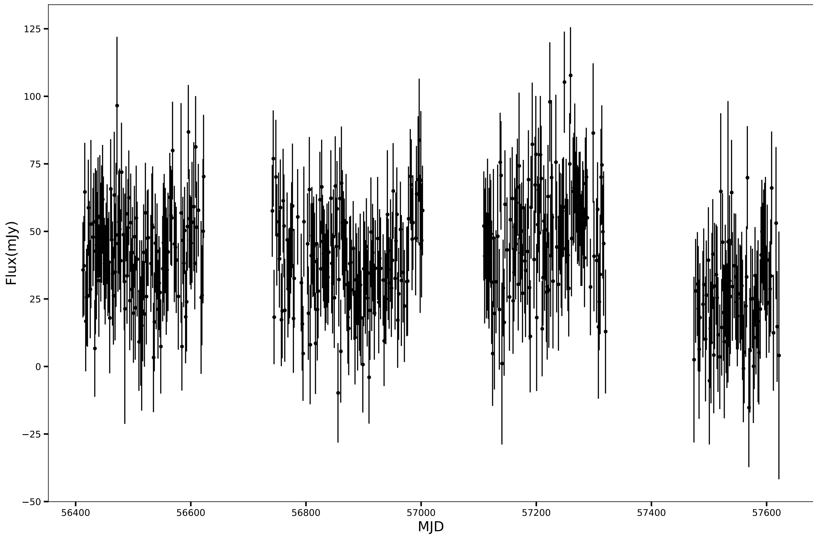
SPT-SJ221015-5031.1, RA=332.5662d, DEC=-50.5188d, mean_flux=39.97 (mJy), 90GHz
