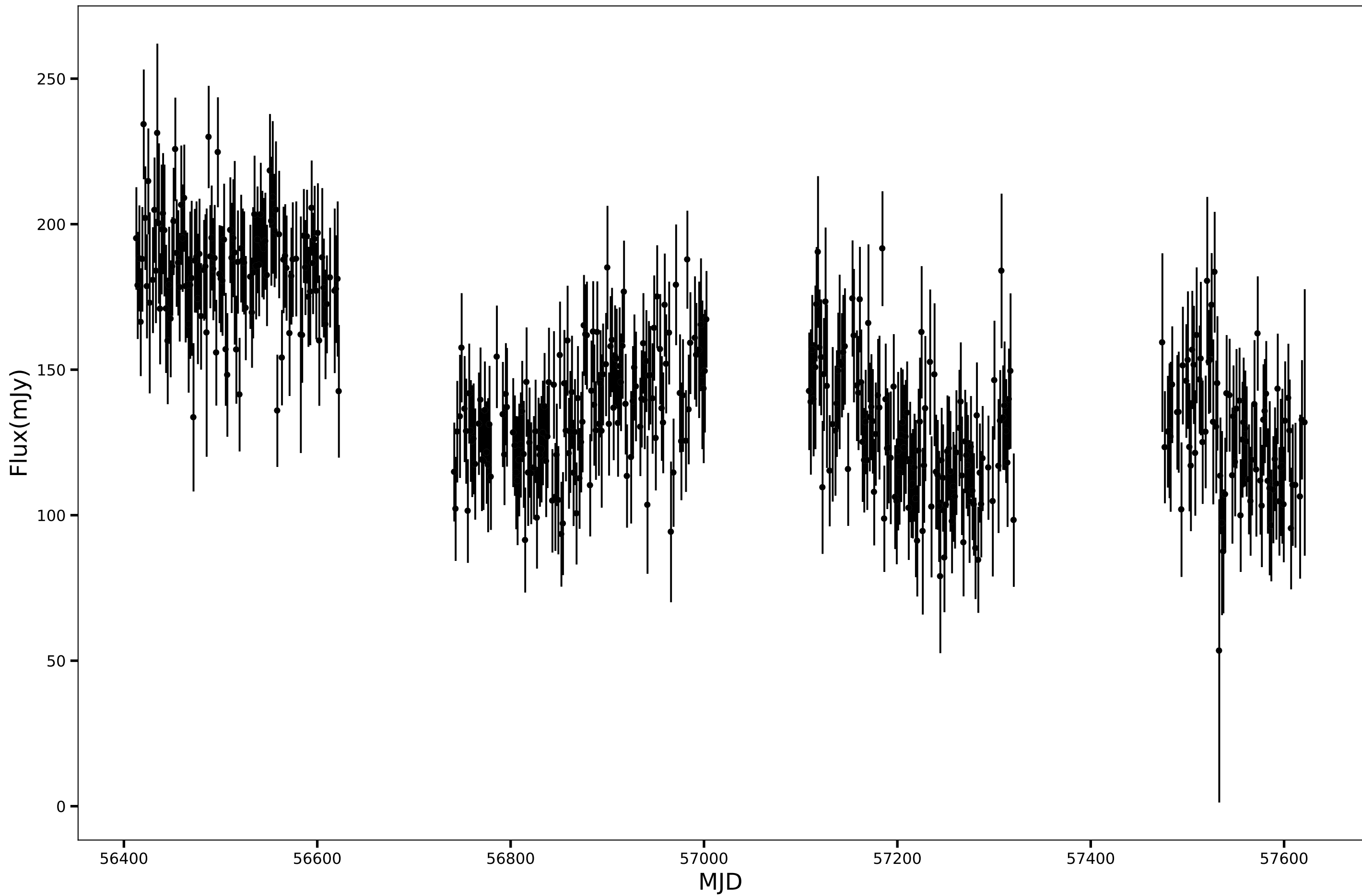
SPT-SJ220846-6325.8, RA=332.1931d, DEC=-63.4304d, mean_flux=145.26 (mJy), 90GHz
