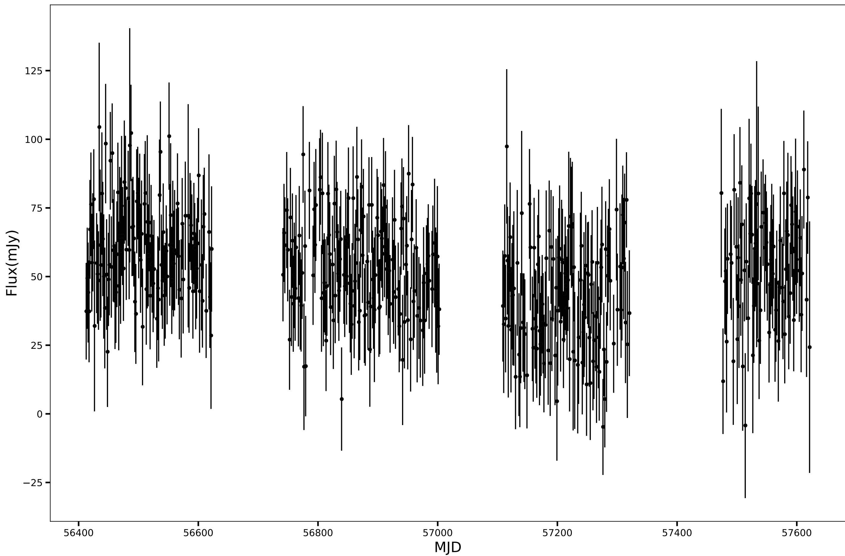
SPT-SJ220715-6325.6, RA=331.8131d, DEC=-63.4280d, mean_flux=51.91 (mJy), 90GHz
