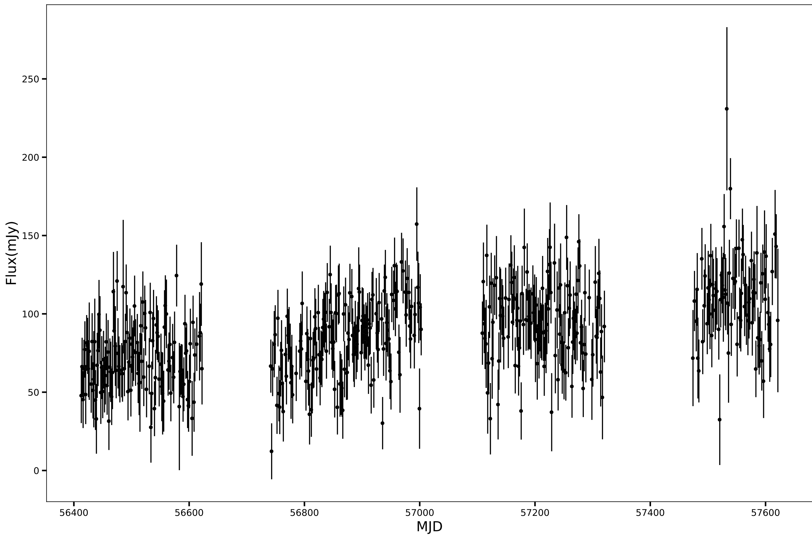
SPT-SJ220301-4937.0, RA=330.7559d, DEC=-49.6173d, mean_flux=87.76 (mJy), 90GHz
