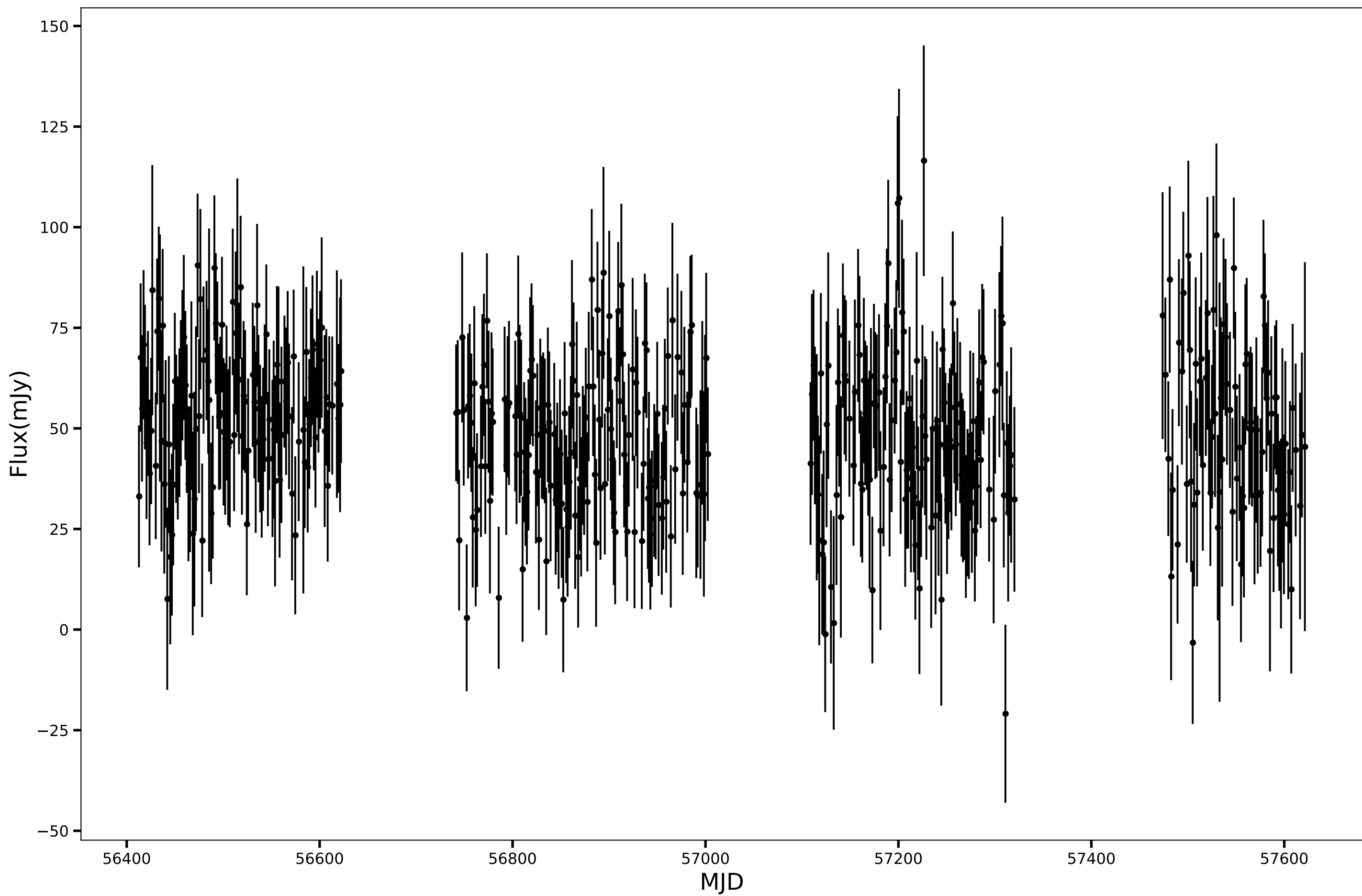
SPT-SJ220253-5635.7, RA=330.7210d, DEC=-56.5953d, mean_flux=49.33 (mJy), 90GHz
