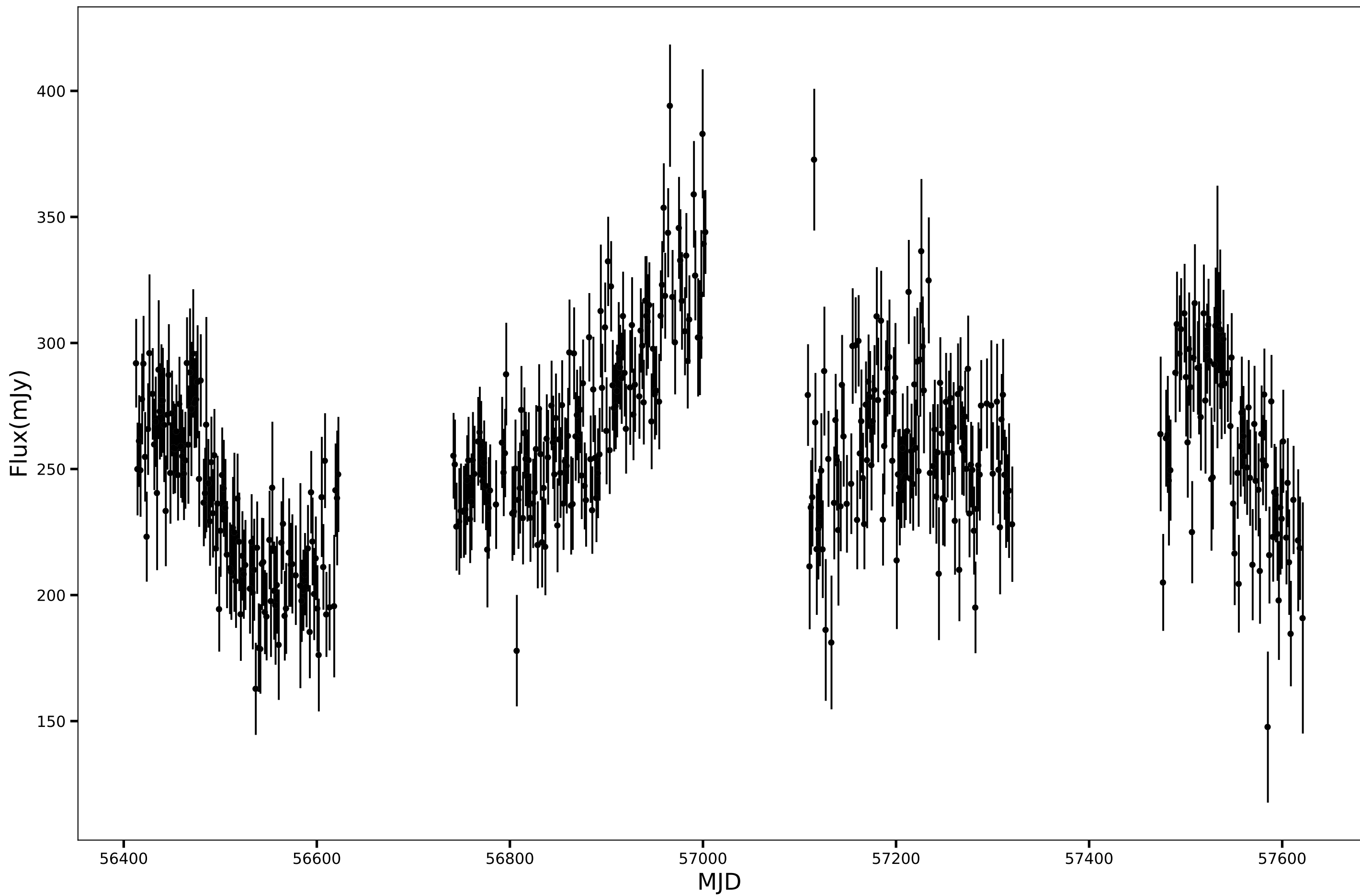
SPT-SJ220055-5520.1, RA=330.2306d, DEC=-55.3356d, mean_flux=256.73 (mJy), 90GHz
