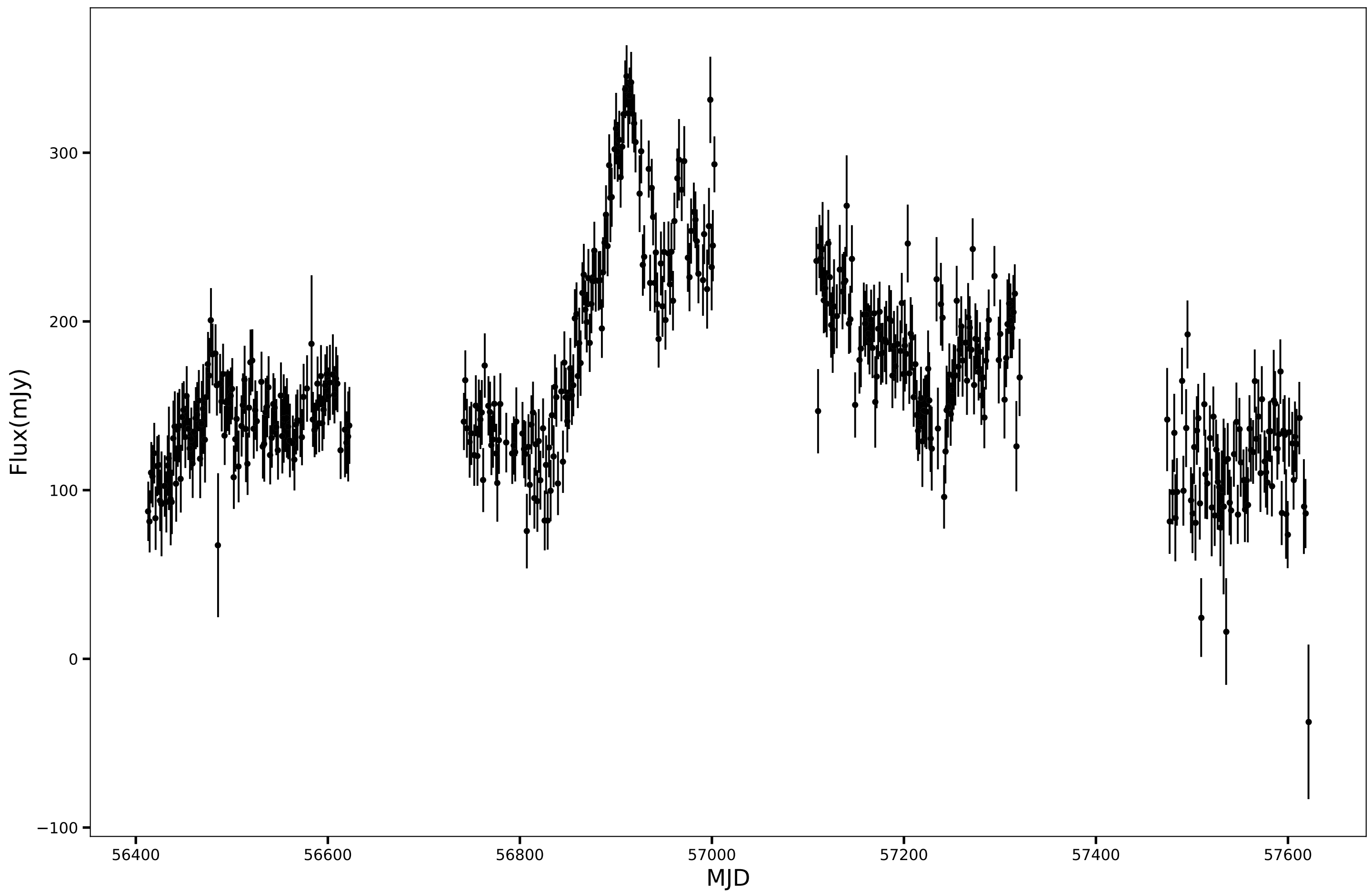
SPT-SJ220005-5455.7, RA=330.0227d, DEC=-54.9290d, mean_flux=165.60 (mJy), 90GHz
