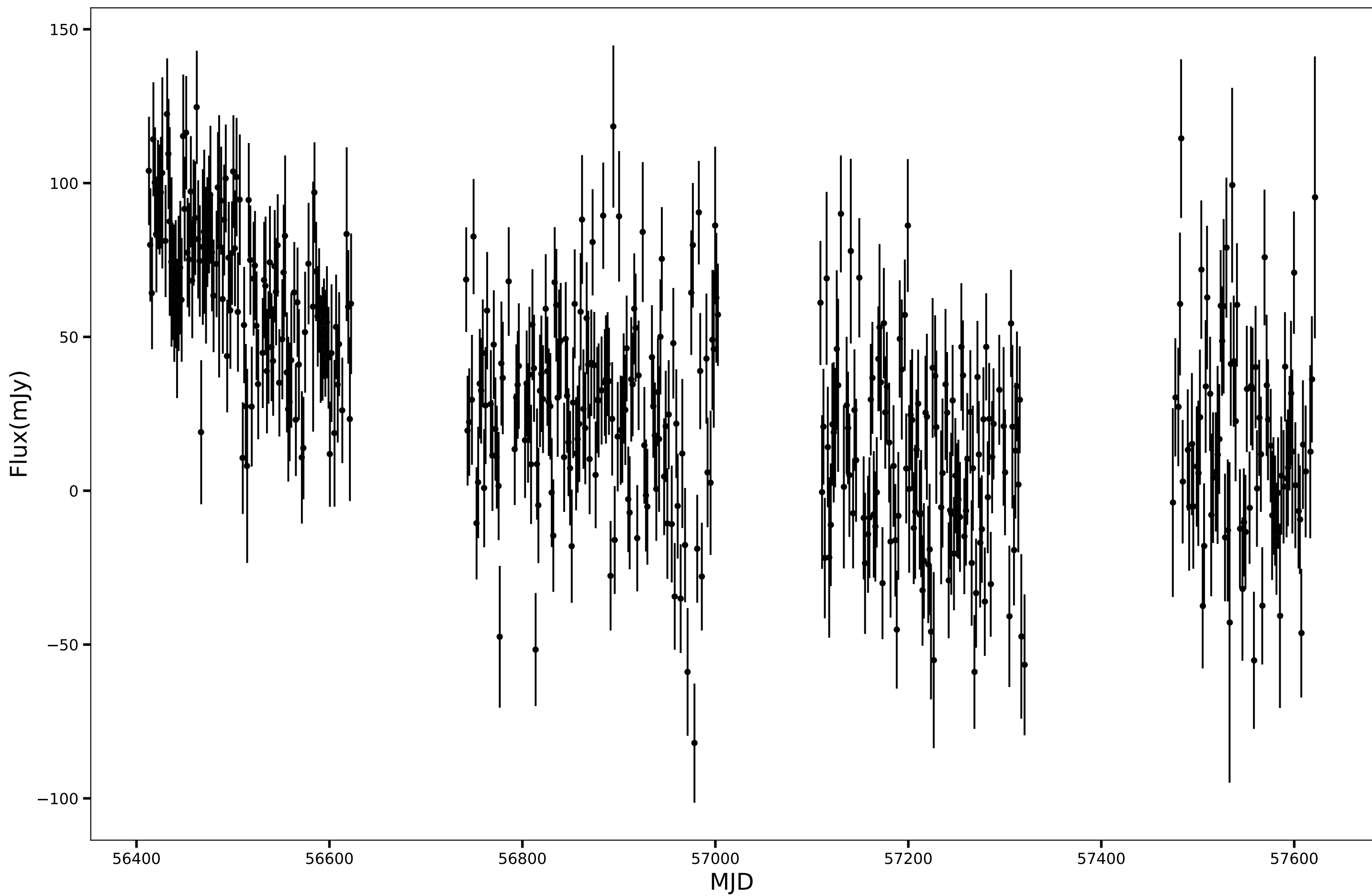
SPT-SJ215648-6331.0, RA=329.2009d, DEC=-63.5179d, mean_flux=30.99 (mJy), 90GHz
