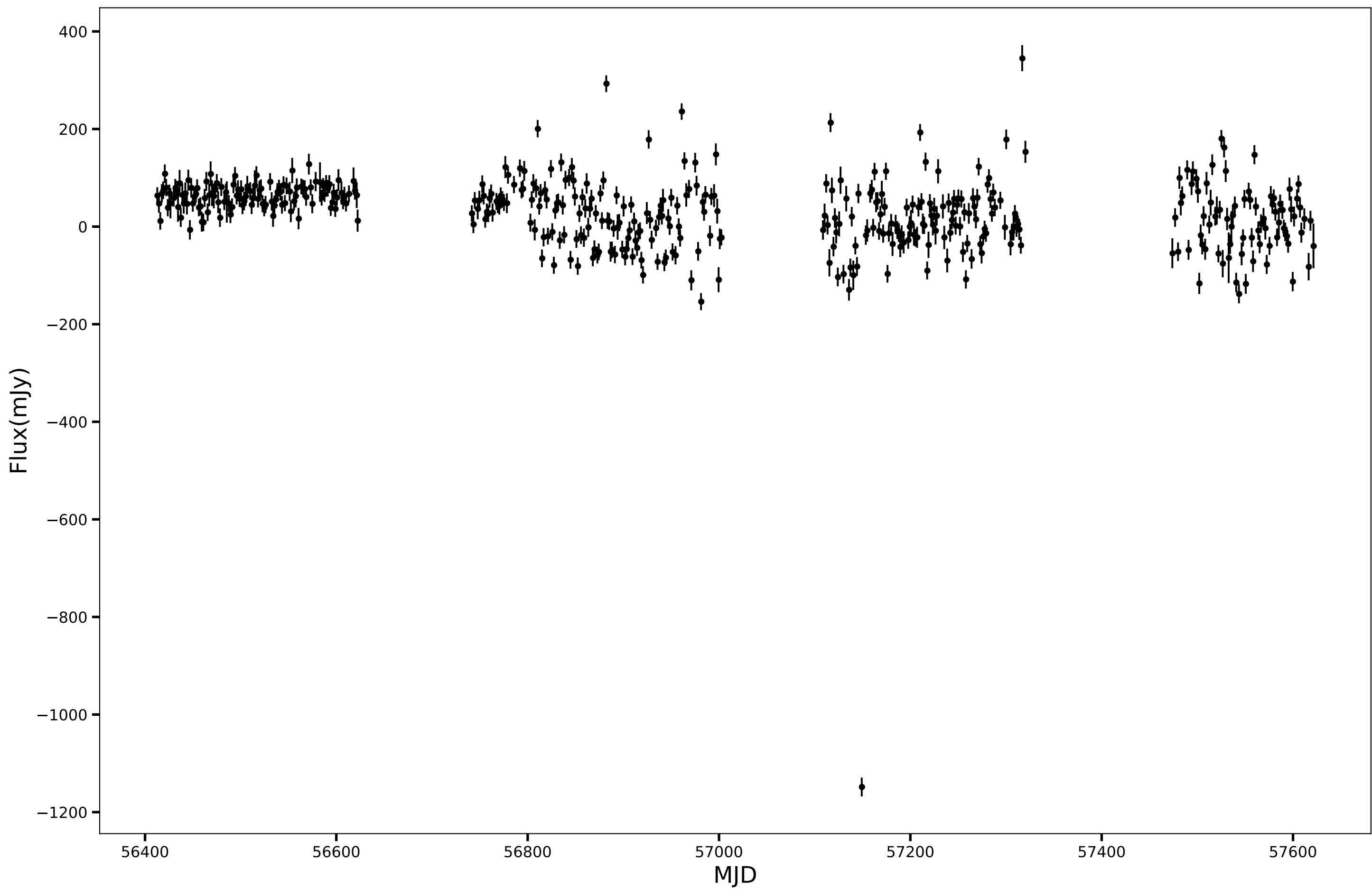
SPT-SJ215445-5725.6, RA=328.6913d, DEC=-57.4277d, mean_flux=28.45 (mJy), 90GHz
