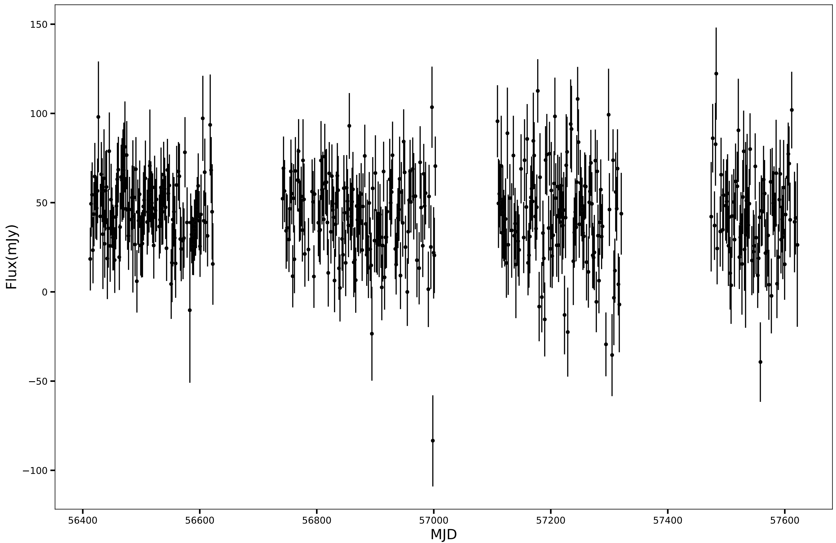
SPT-SJ015853-6334.8, RA=29.7244d, DEC=-63.5801d, mean_flux=43.35 (mJy), 90GHz
