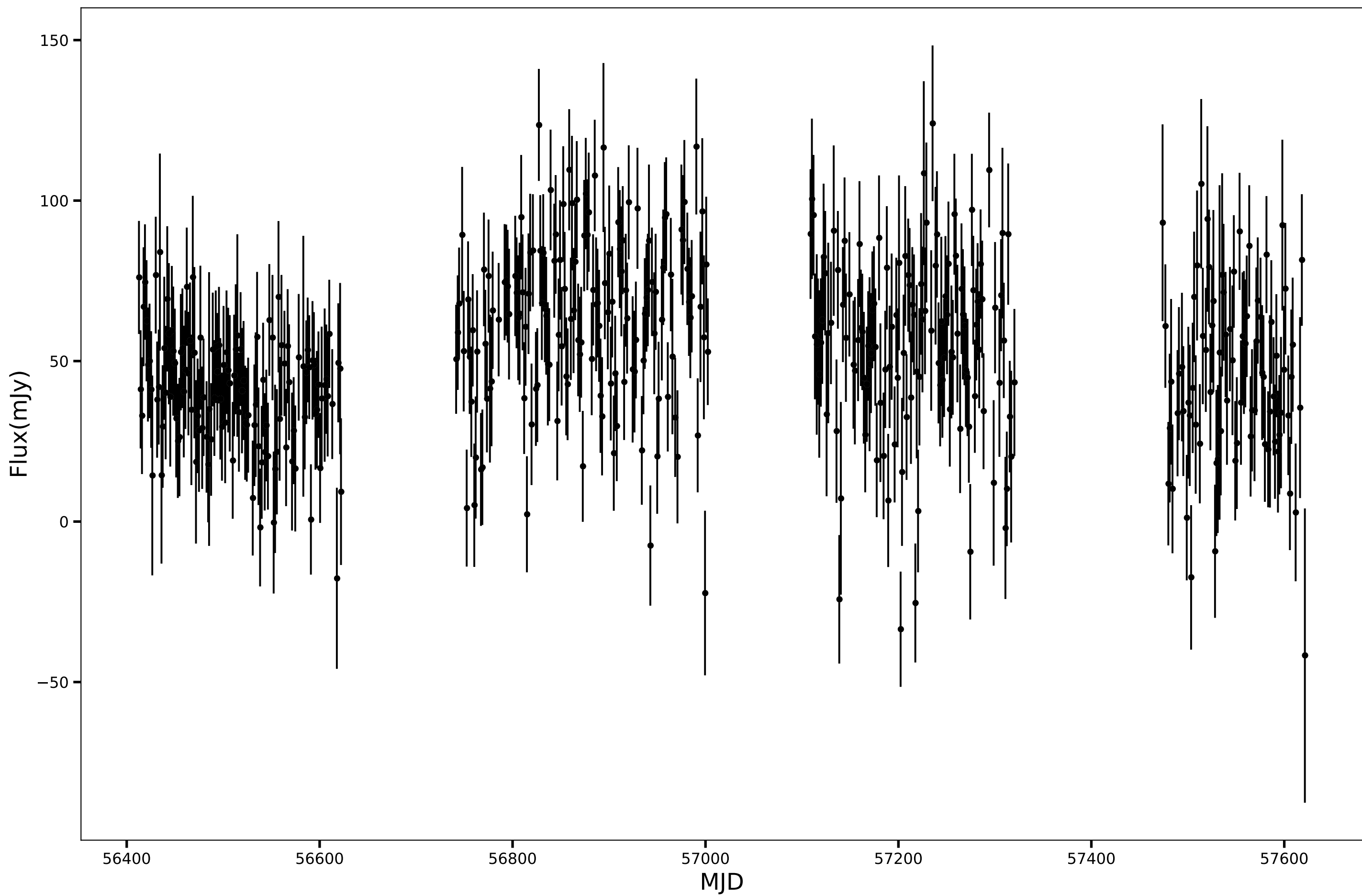
SPT-SJ015838-6419.3, RA=29.6592d, DEC=-64.3224d, mean_flux=52.18 (mJy), 90GHz
