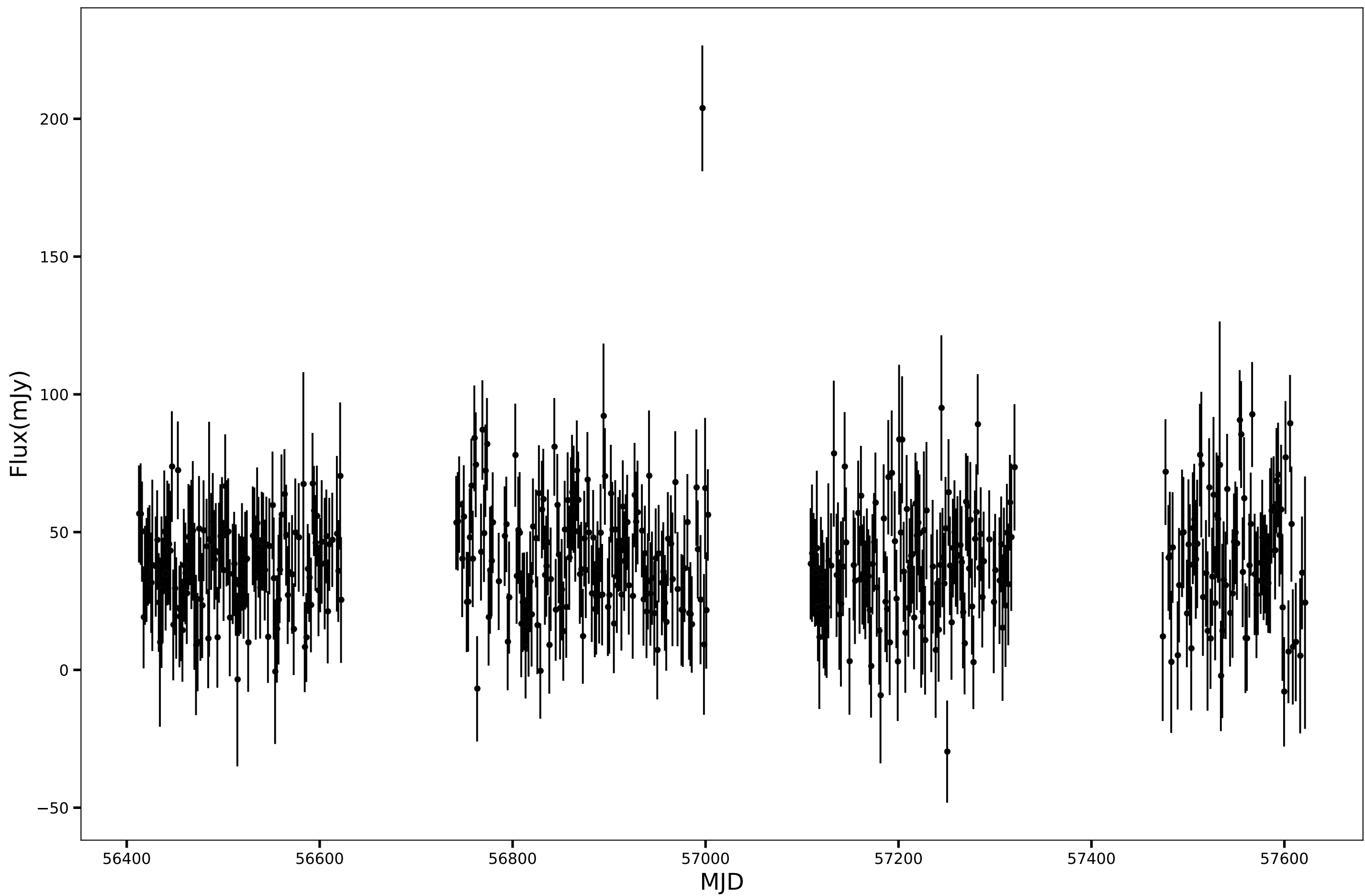
SPT-SJ015816-5004.3, RA=29.5677d, DEC=-50.0732d, mean_flux=39.60 (mJy), 90GHz
