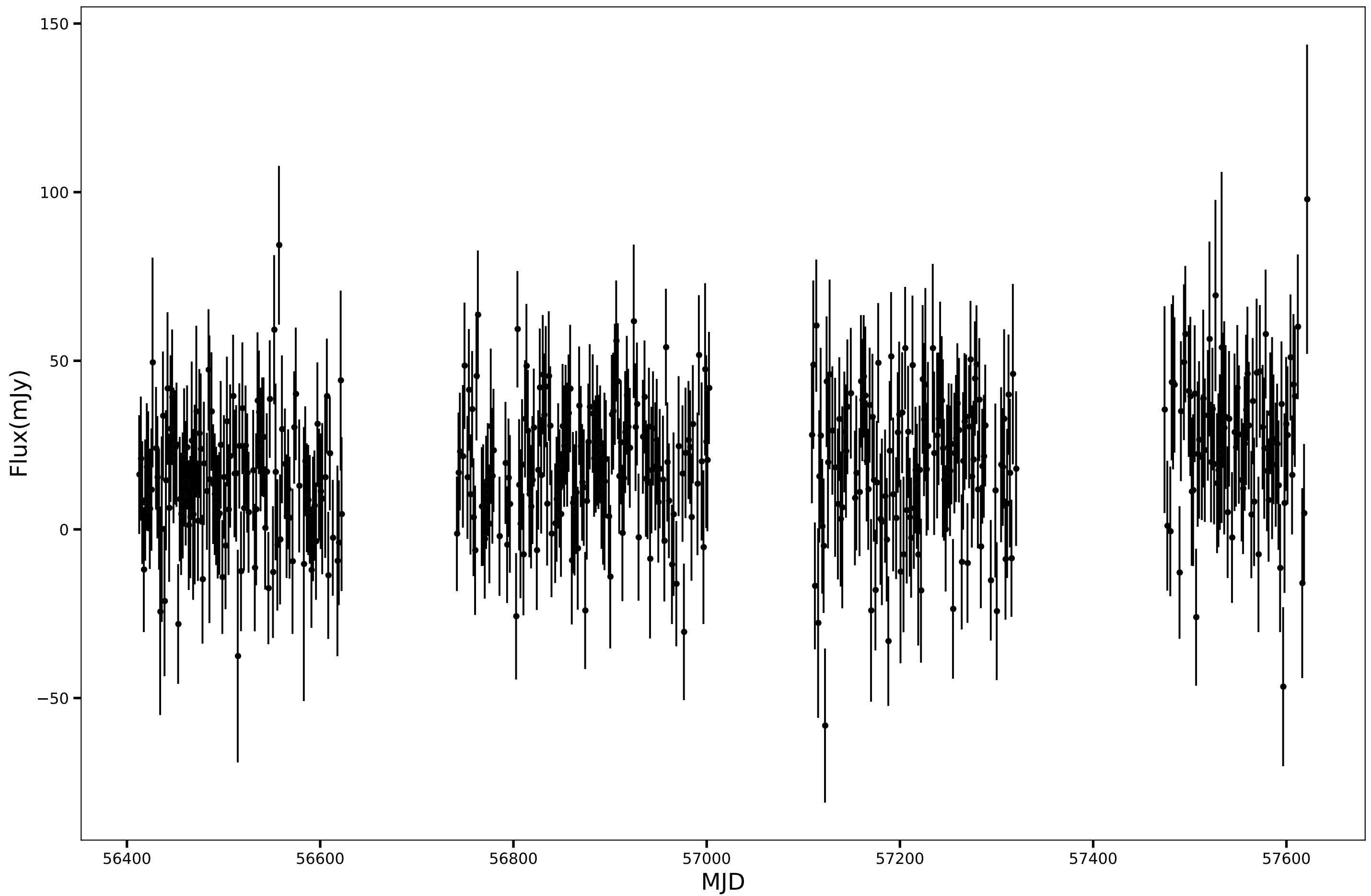
SPT-SJ015721-5422.6, RA=29.3398d, DEC=-54.3774d, mean_flux=18.97 (mJy), 90GHz
