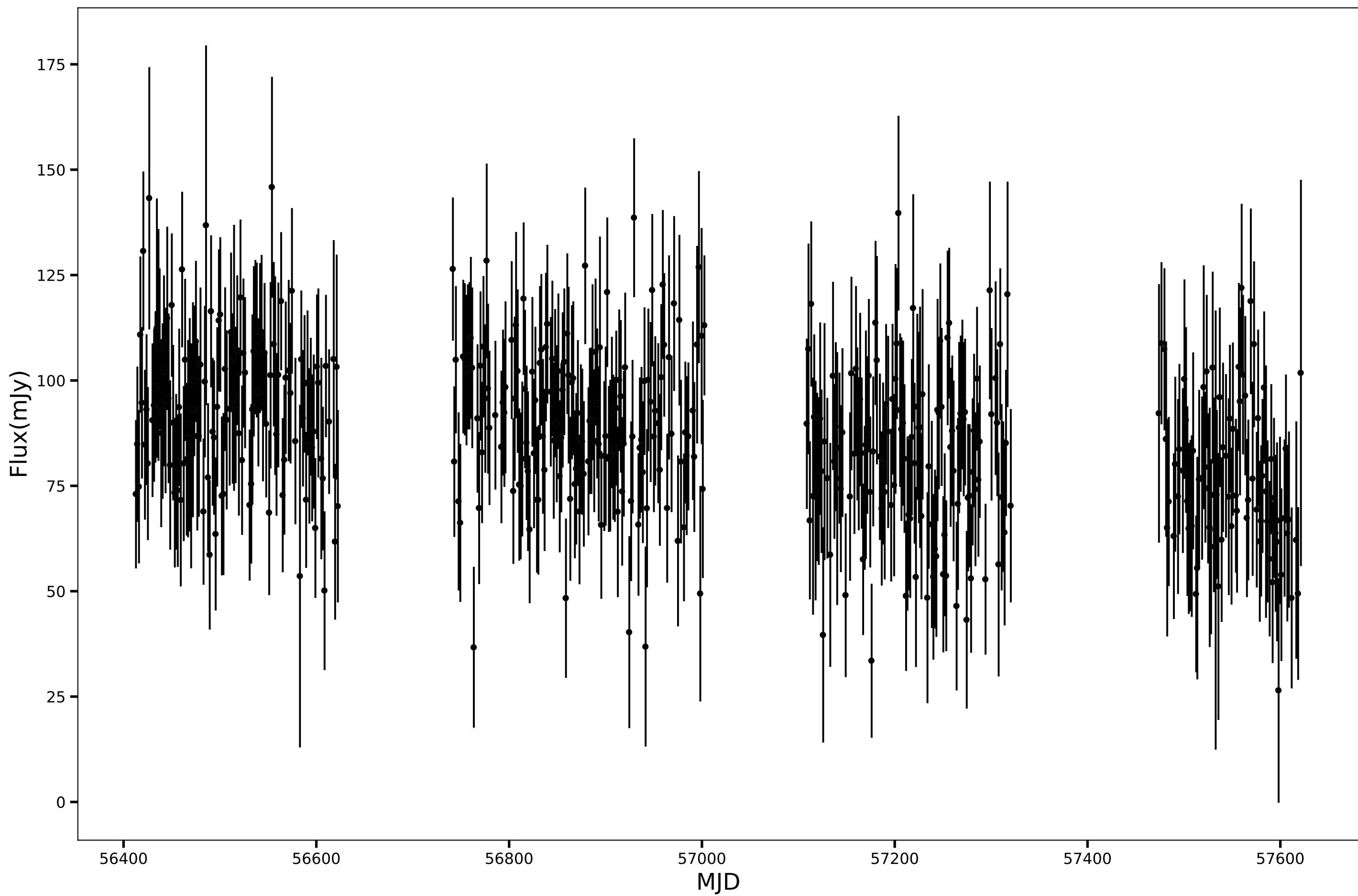
SPT-SJ015650-5439.7, RA=29.2110d, DEC=-54.6620d, mean_flux=86.94 (mJy), 90GHz
