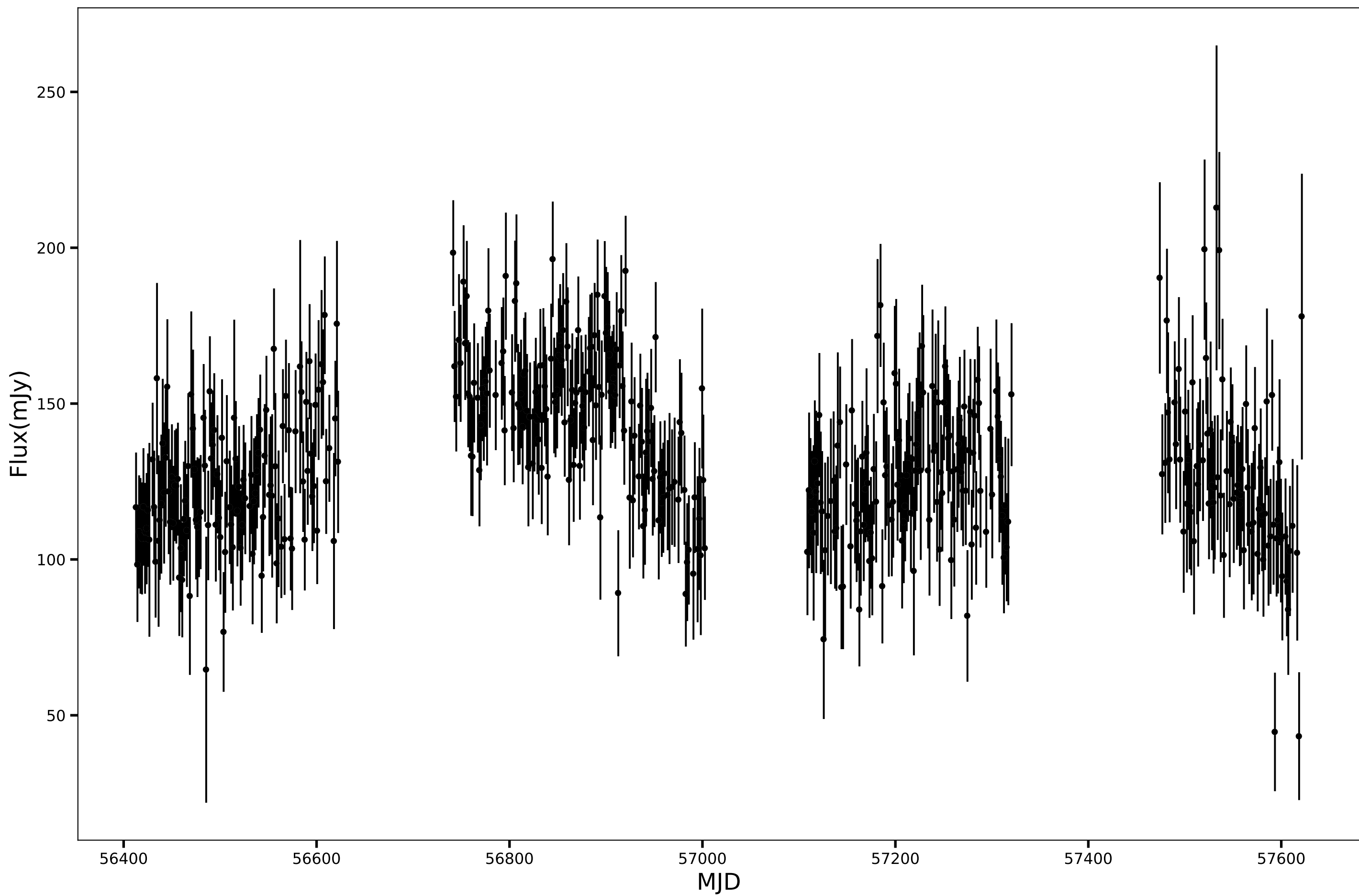
SPT-SJ015419-5107.9, RA=28.5819d, DEC=-51.1326d, mean_flux=132.11 (mJy), 90GHz
