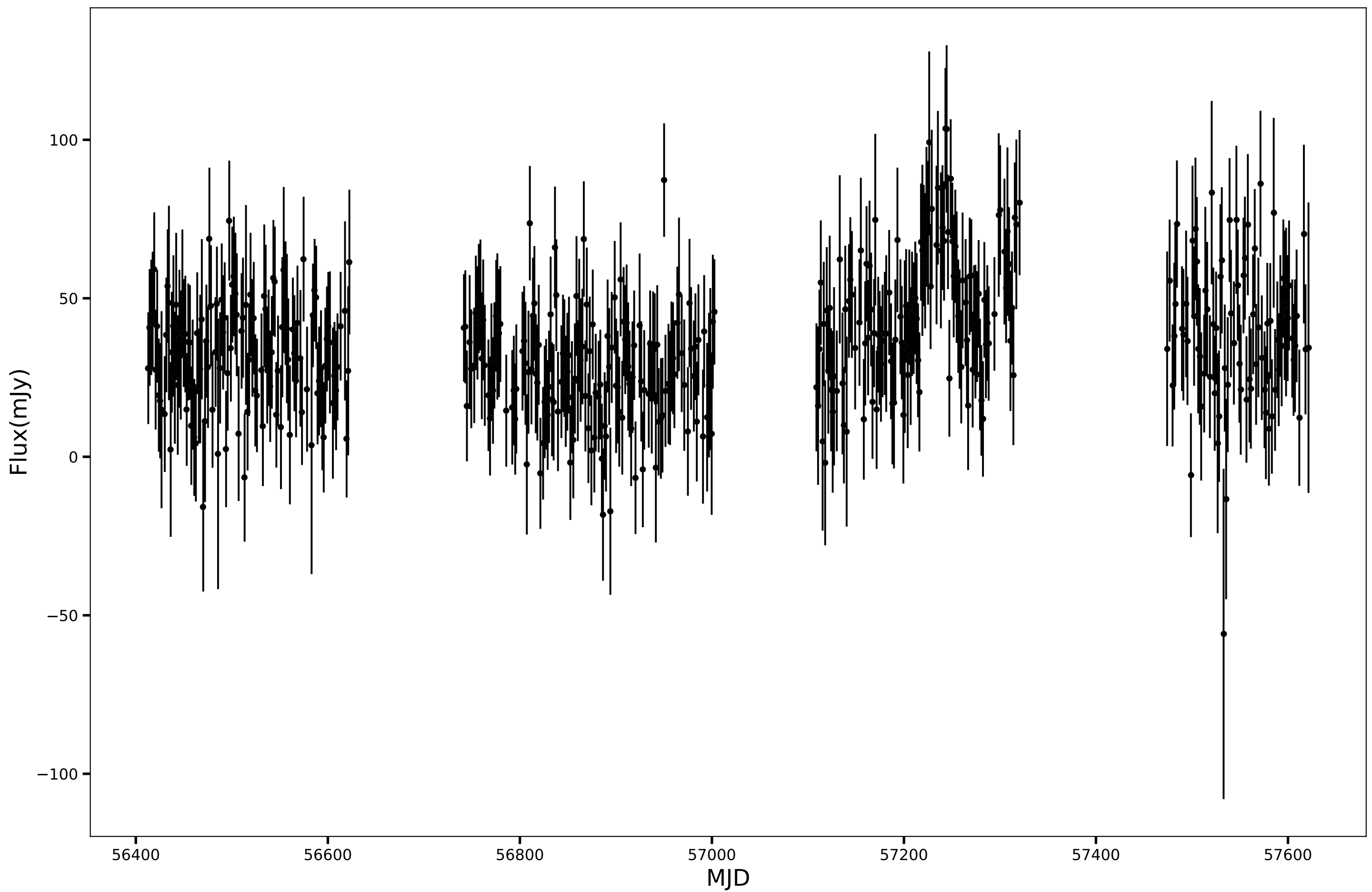
SPT-SJ015050-6044.2, RA=27.7096d, DEC=-60.7368d, mean_flux=35.29 (mJy), 90GHz
