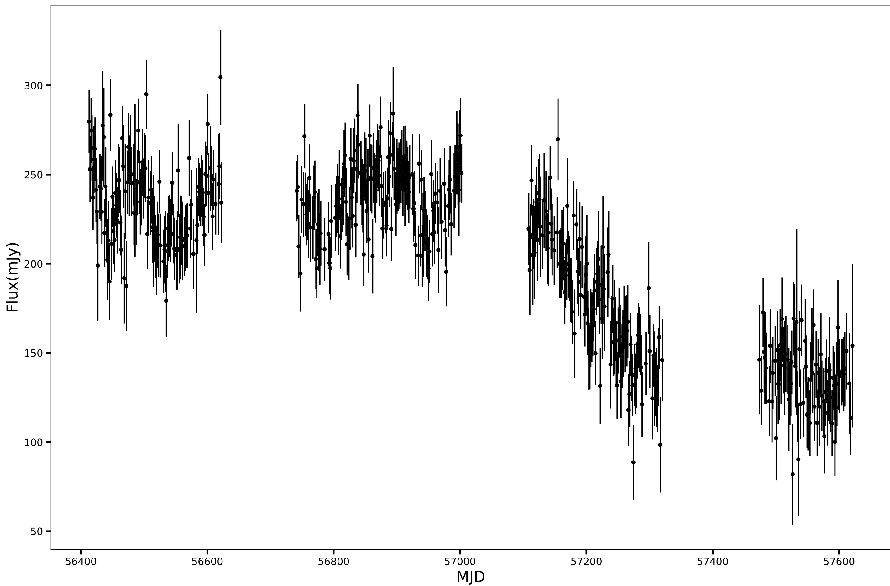
SPT-SJ014415-6421.8, RA=26.0657d, DEC=-64.3648d, mean_flux=203.57 (mJy), 90GHz
