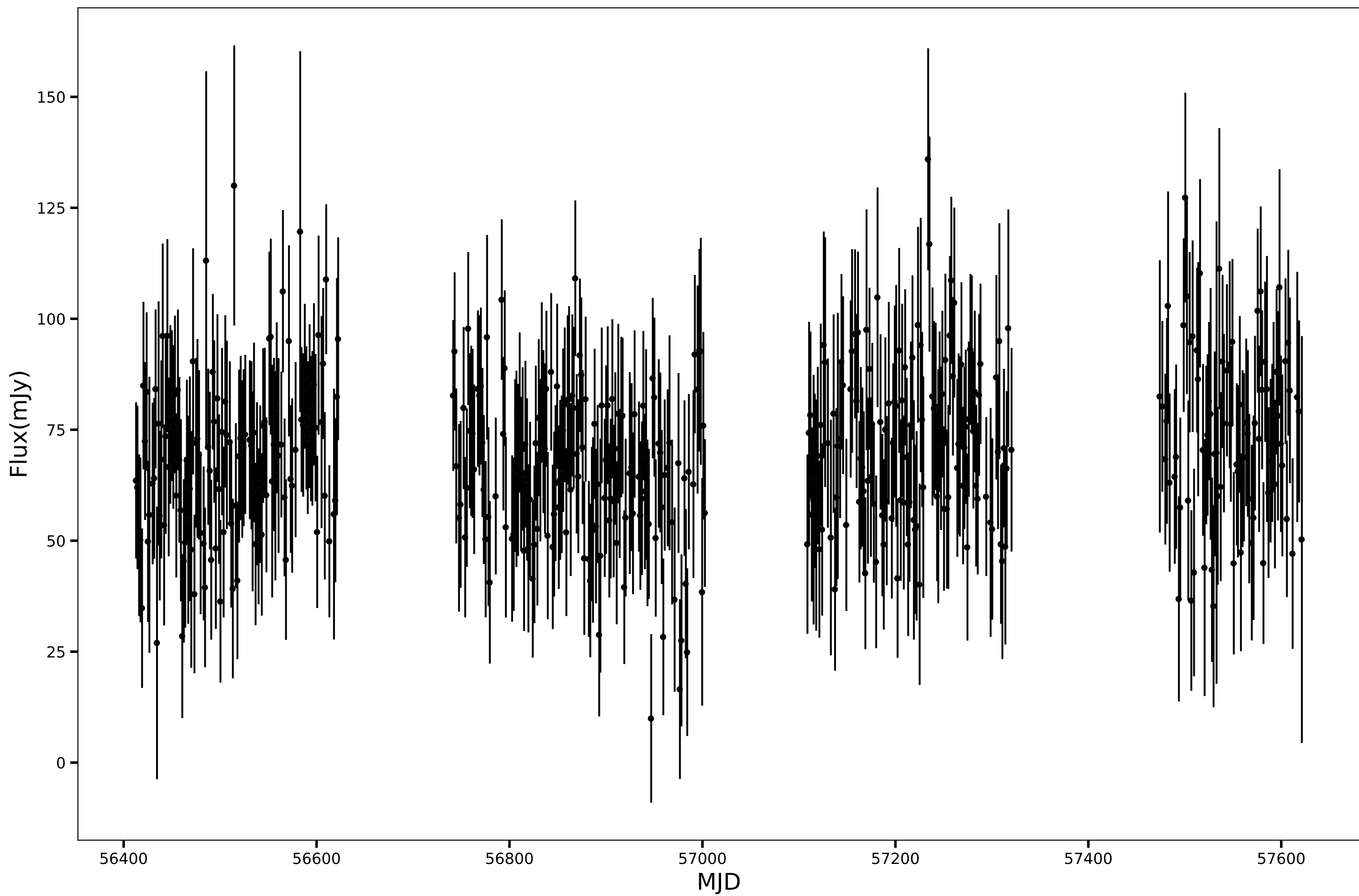
SPT-SJ014257-6044.9, RA=25.7376d, DEC=-60.7498d, mean_flux=69.64 (mJy), 90GHz
