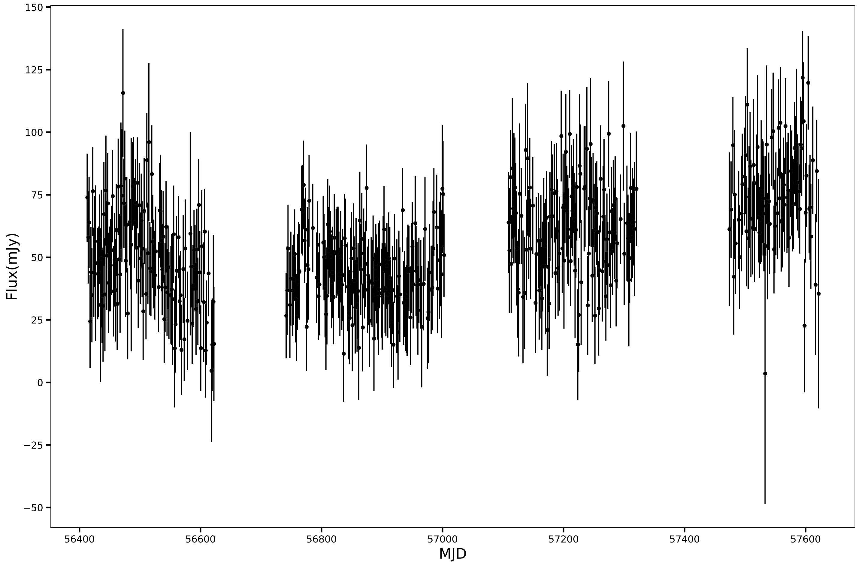
SPT-SJ014142-5650.6, RA=25.4274d, DEC=-56.8442d, mean_flux=54.63 (mJy), 90GHz
