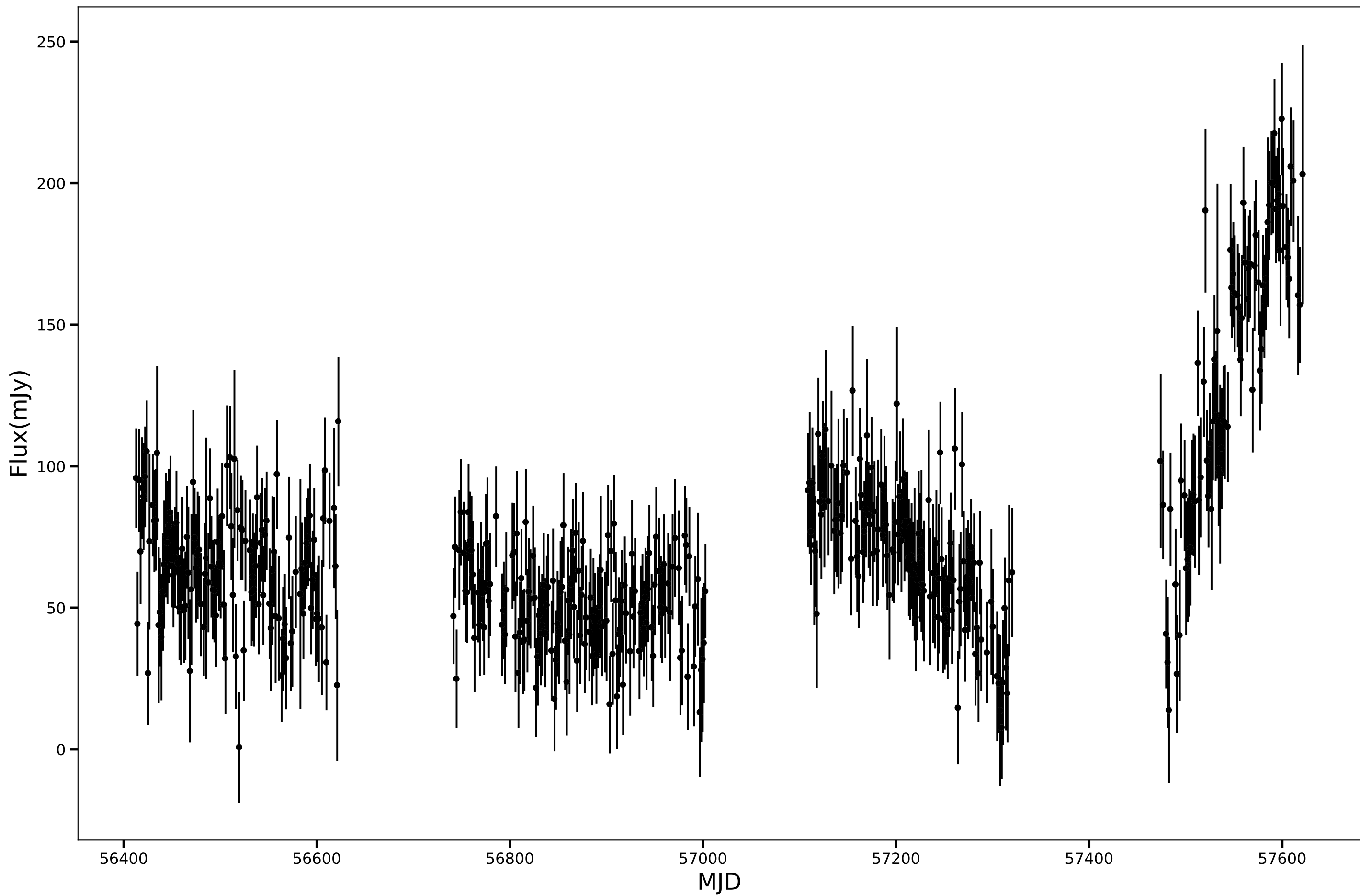
SPT-SJ013949-5217.7, RA=24.9547d, DEC=-52.2963d, mean_flux=73.79 (mJy), 90GHz
