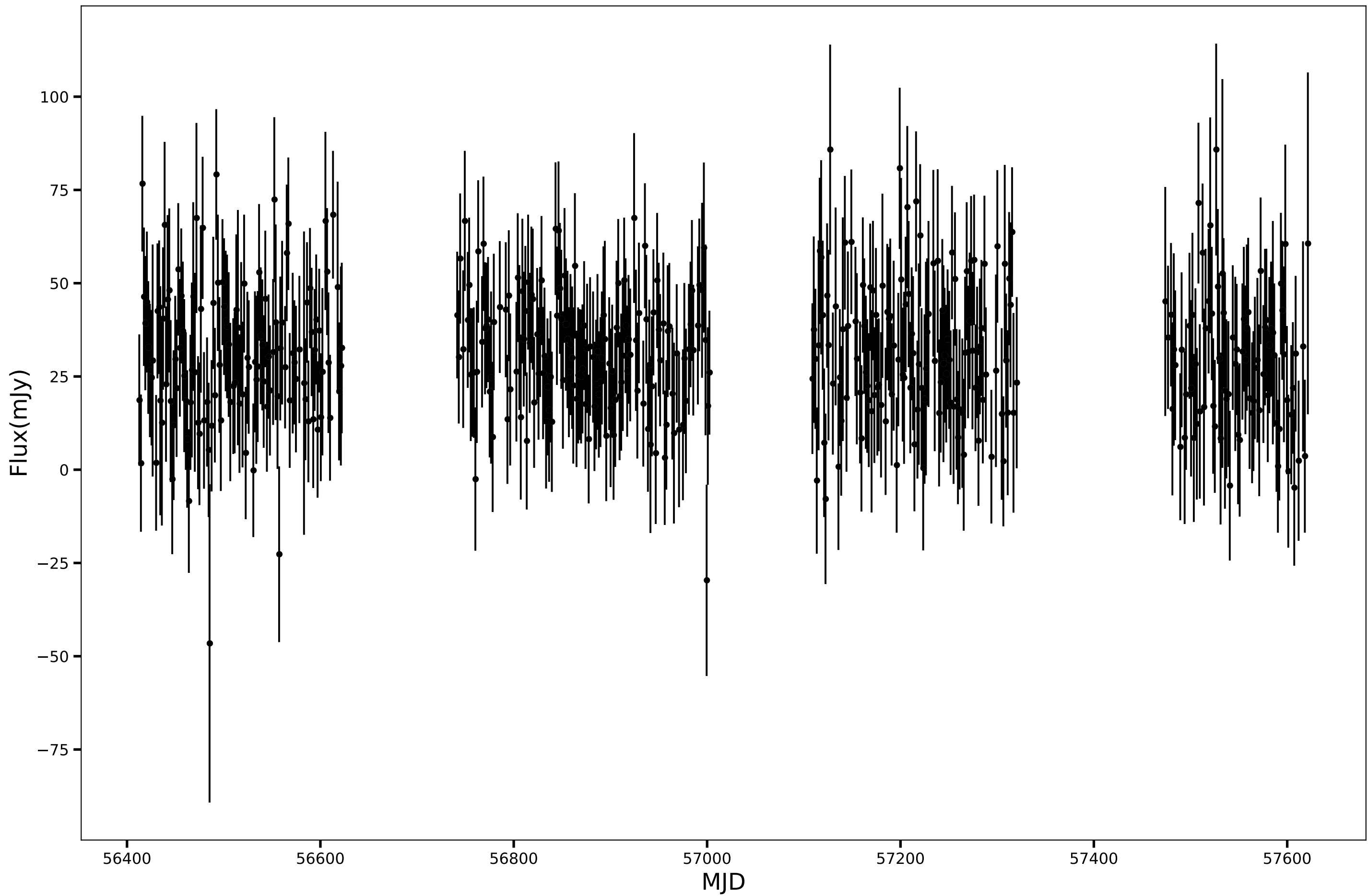
SPT-SJ013540-5149.7, RA=23.9183d, DEC=-51.8291d, mean_flux=30.98 (mJy), 90GHz
