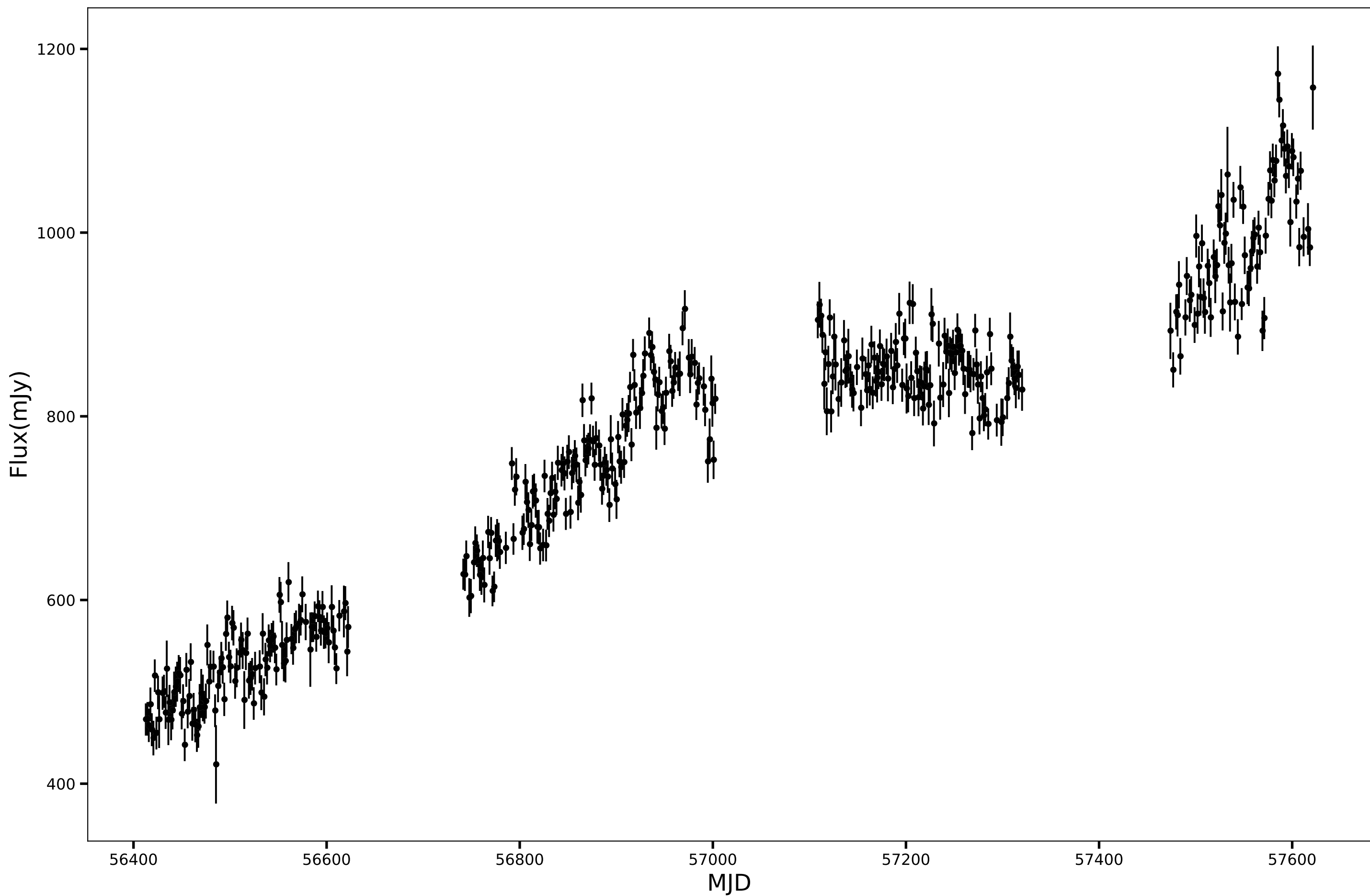
SPT-SJ013305-5200.1, RA=23.2711d, DEC=-52.0018d, mean_flux=759.08 (mJy), 90GHz
