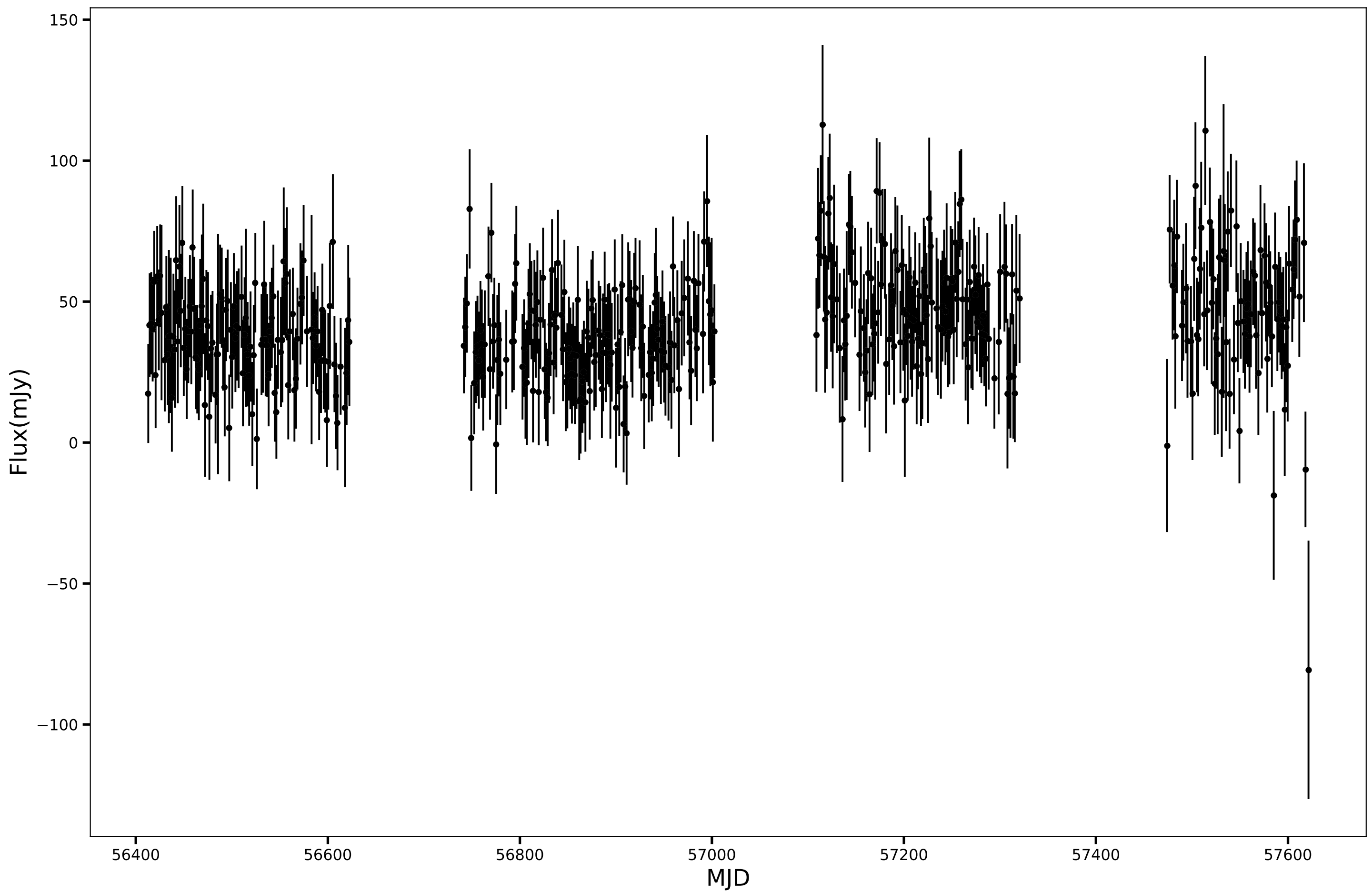
SPT-SJ012755-5136.6, RA=21.9807d, DEC=-51.6109d, mean_flux=41.81 (mJy), 90GHz
