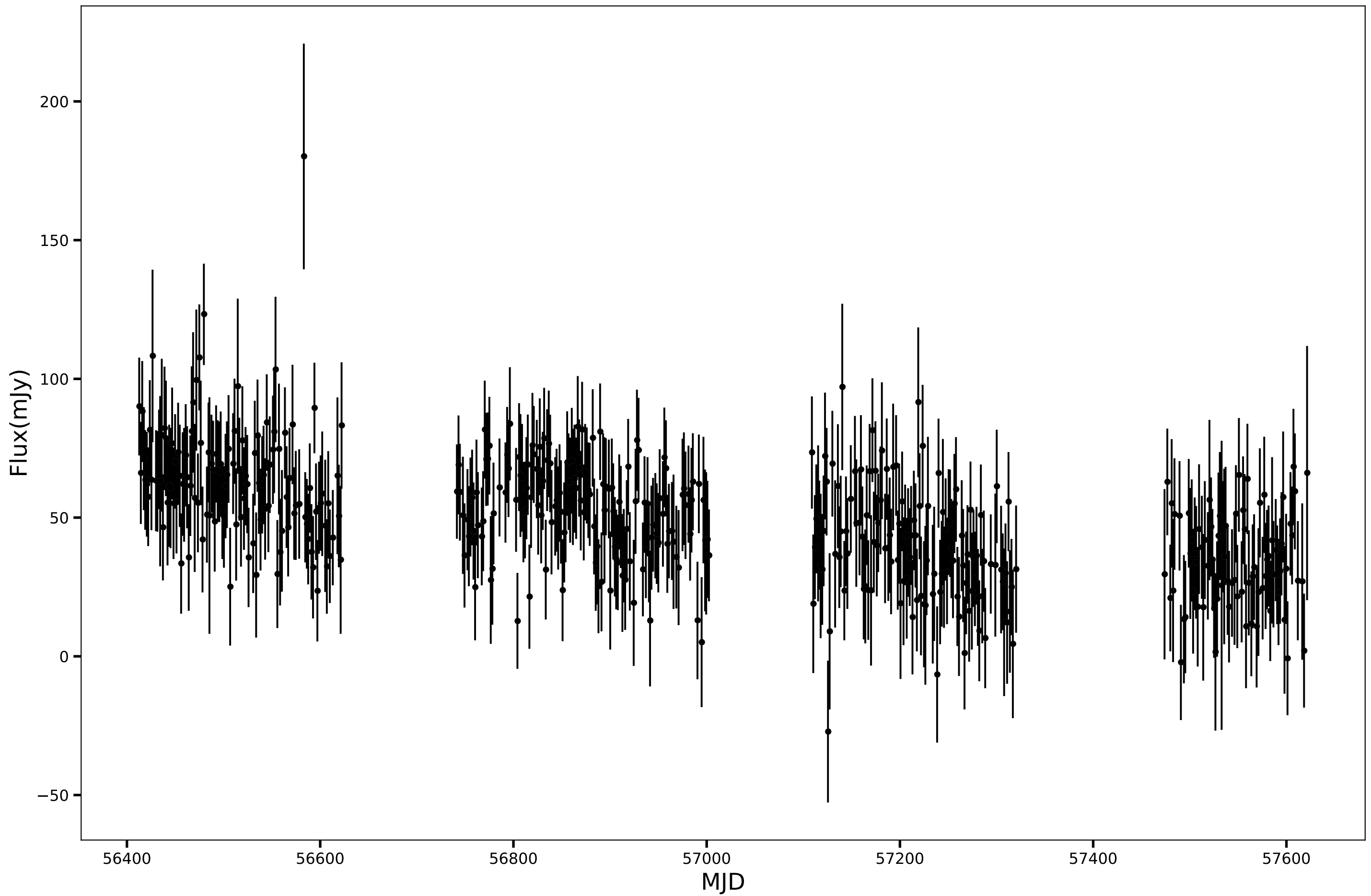
SPT-SJ012140-6309.2, RA=20.4188d, DEC=-63.1536d, mean_flux=48.90 (mJy), 90GHz
