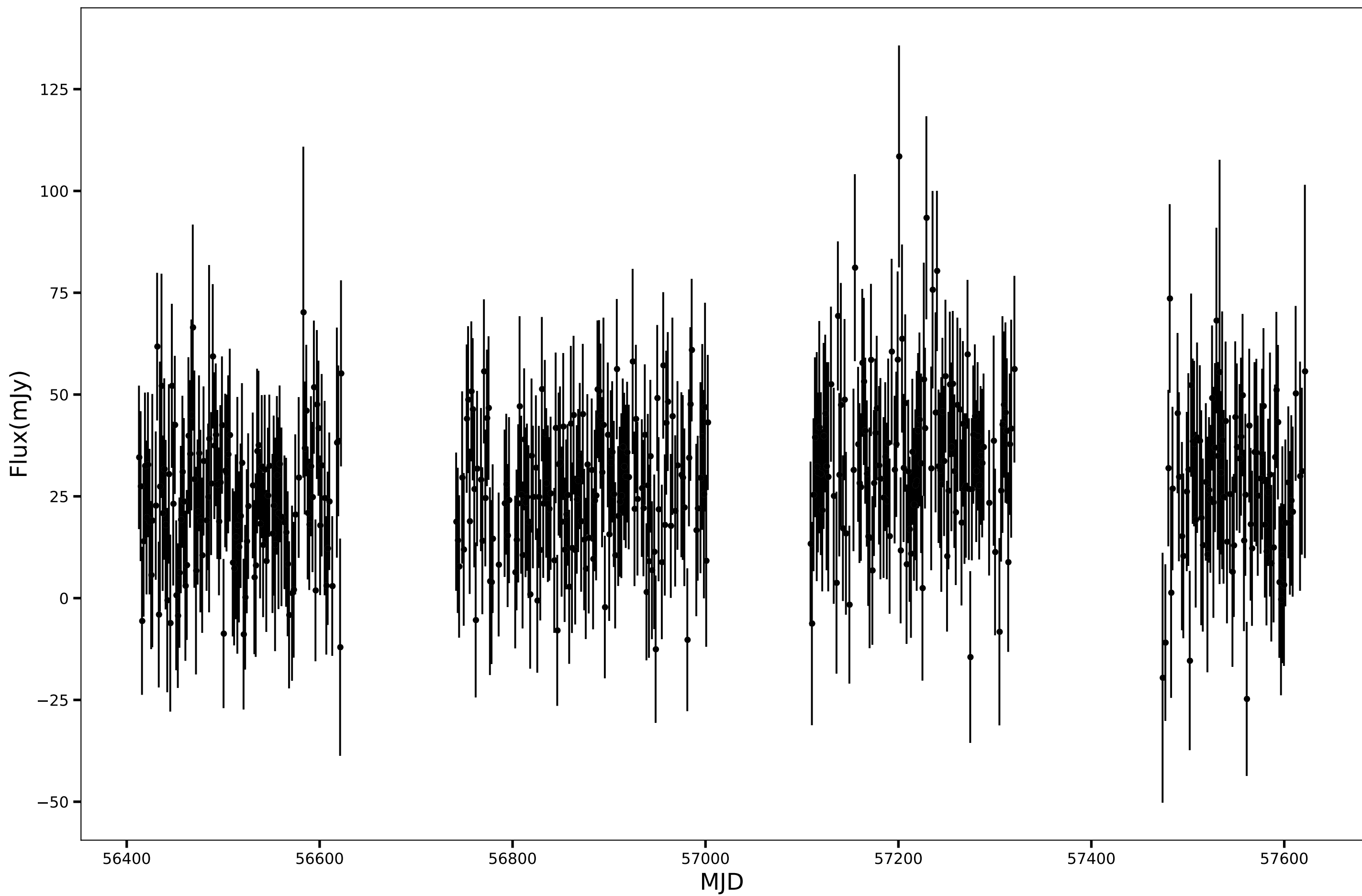
SPT-SJ012007-5211.1, RA=20.0314d, DEC=-52.1858d, mean_flux=28.00 (mJy), 90GHz
