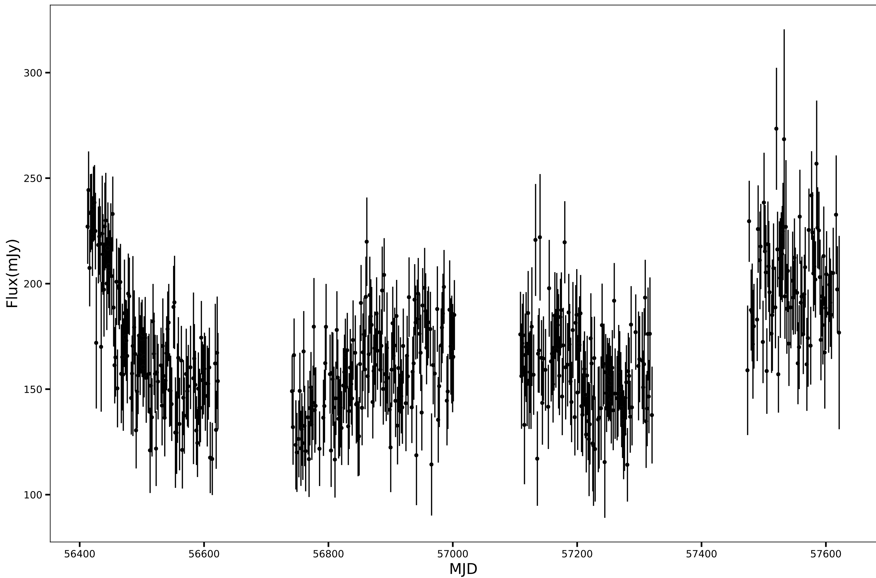
SPT-SJ011950-5357.2, RA=19.9614d, DEC=-53.9546d, mean_flux=168.79 (mJy), 90GHz
