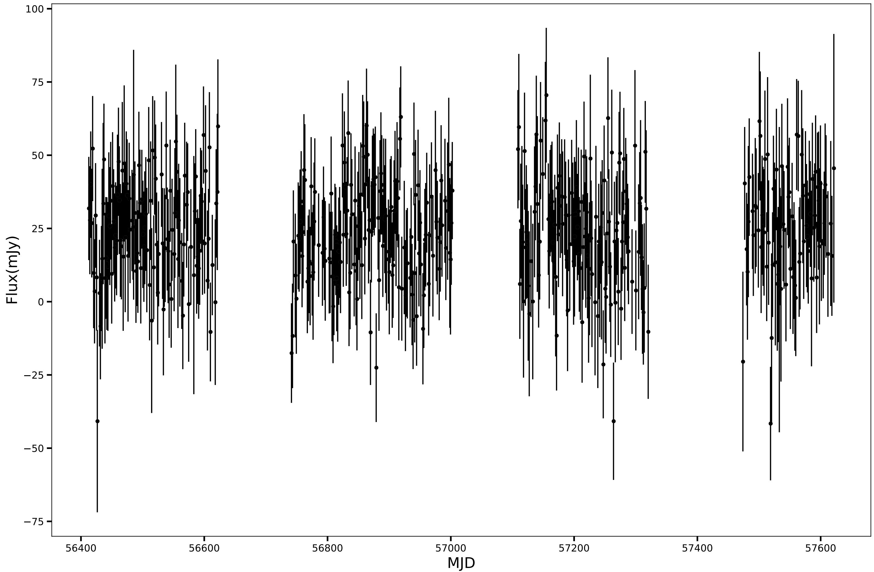
SPT-SJ011323-5329.8, RA=18.3475d, DEC=-53.4973d, mean_flux=23.80 (mJy), 90GHz
