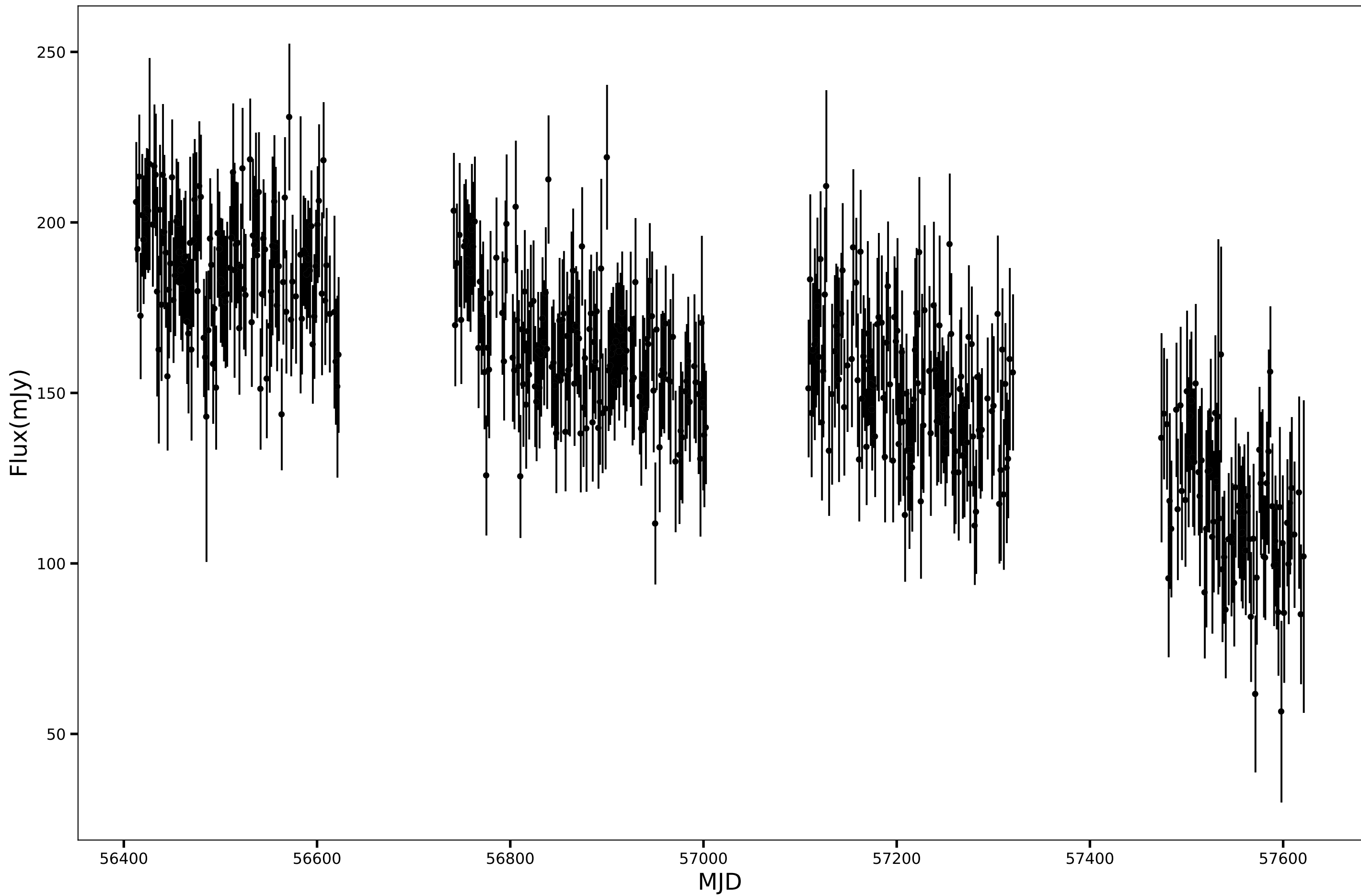
SPT-SJ011016-6316.0, RA=17.5688d, DEC=-63.2669d, mean_flux=158.45 (mJy), 90GHz
