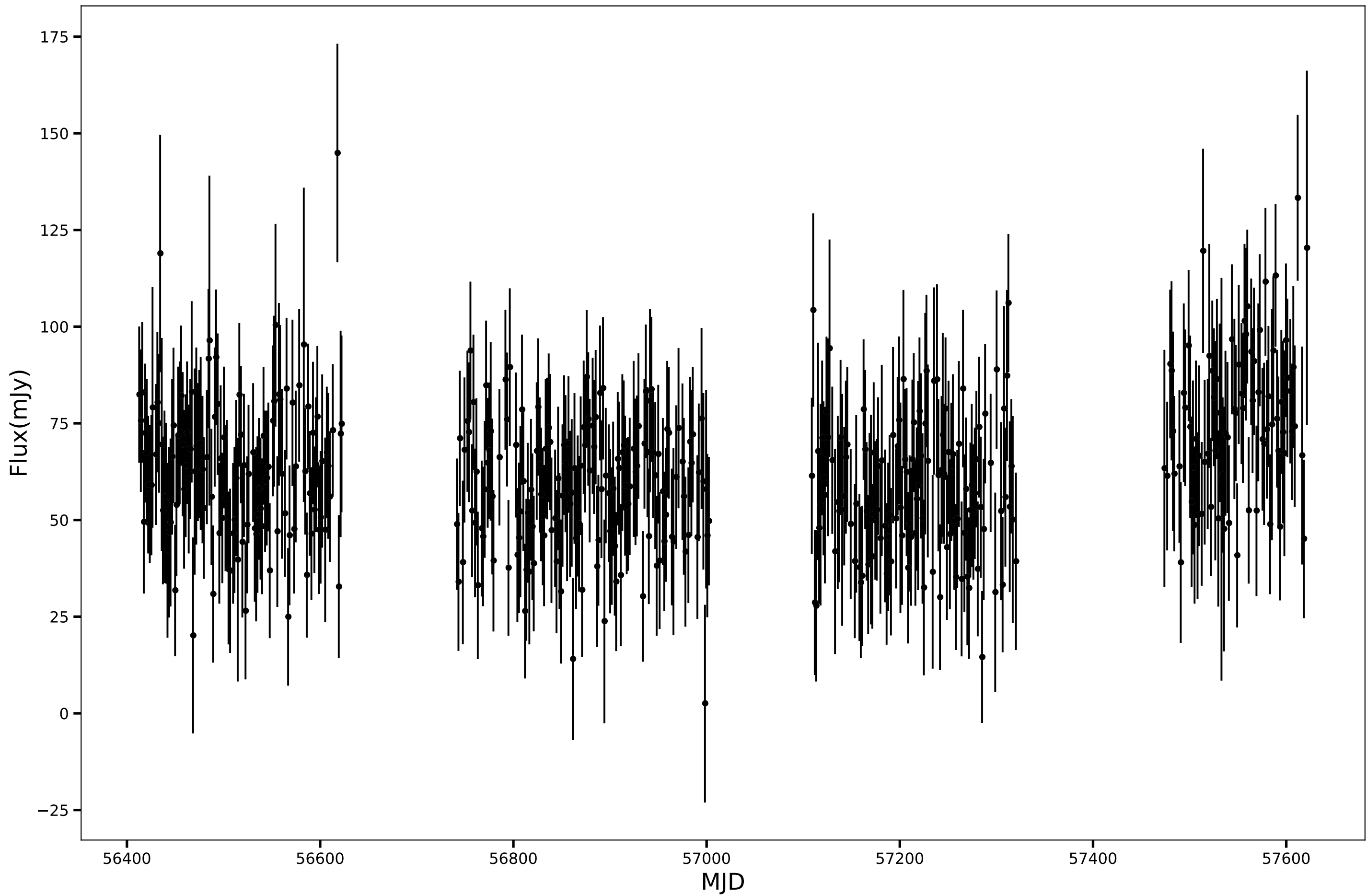
SPT-SJ010406-5657.3, RA=16.0288d, DEC=-56.9554d, mean_flux=62.32 (mJy), 90GHz
