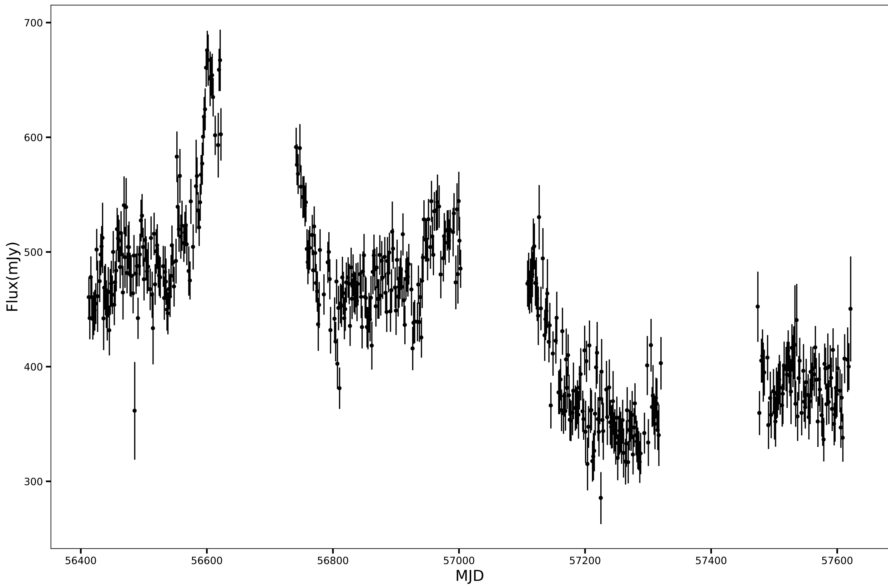
SPT-SJ010333-6439.2, RA=15.8895d, DEC=-64.6536d, mean_flux=446.29 (mJy), 90GHz
