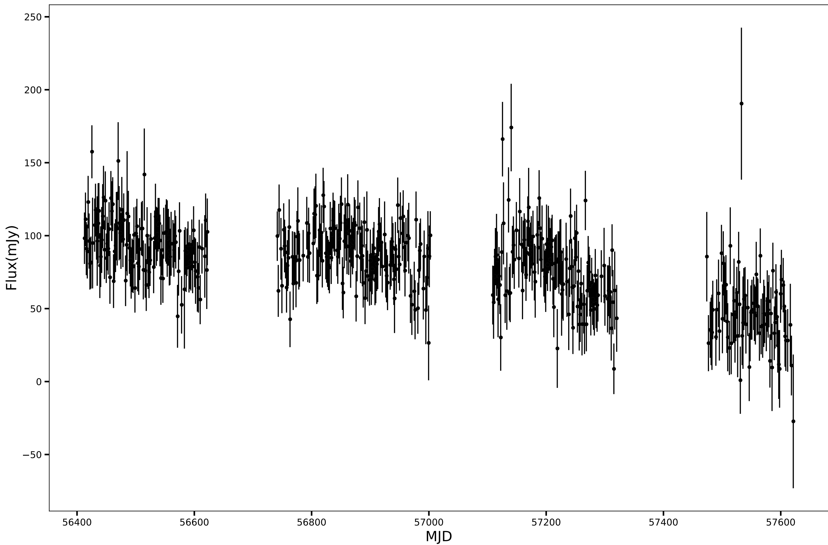
SPT-SJ010306-5109.1, RA=15.7758d, DEC=-51.1525d, mean_flux=79.37 (mJy), 90GHz
