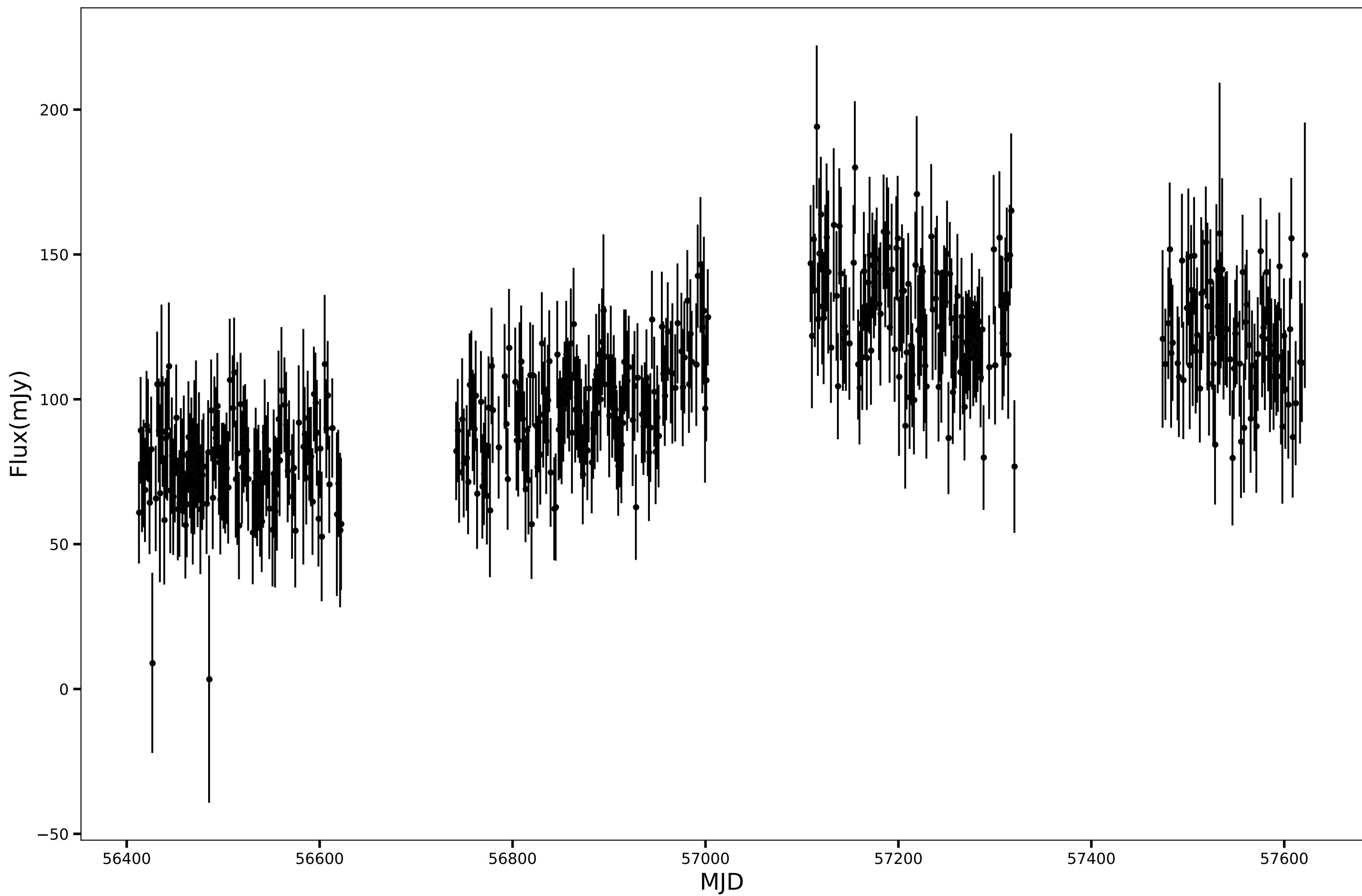
SPT-SJ010115-6233.2, RA=15.3127d, DEC=-62.5533d, mean_flux=104.74 (mJy), 90GHz
