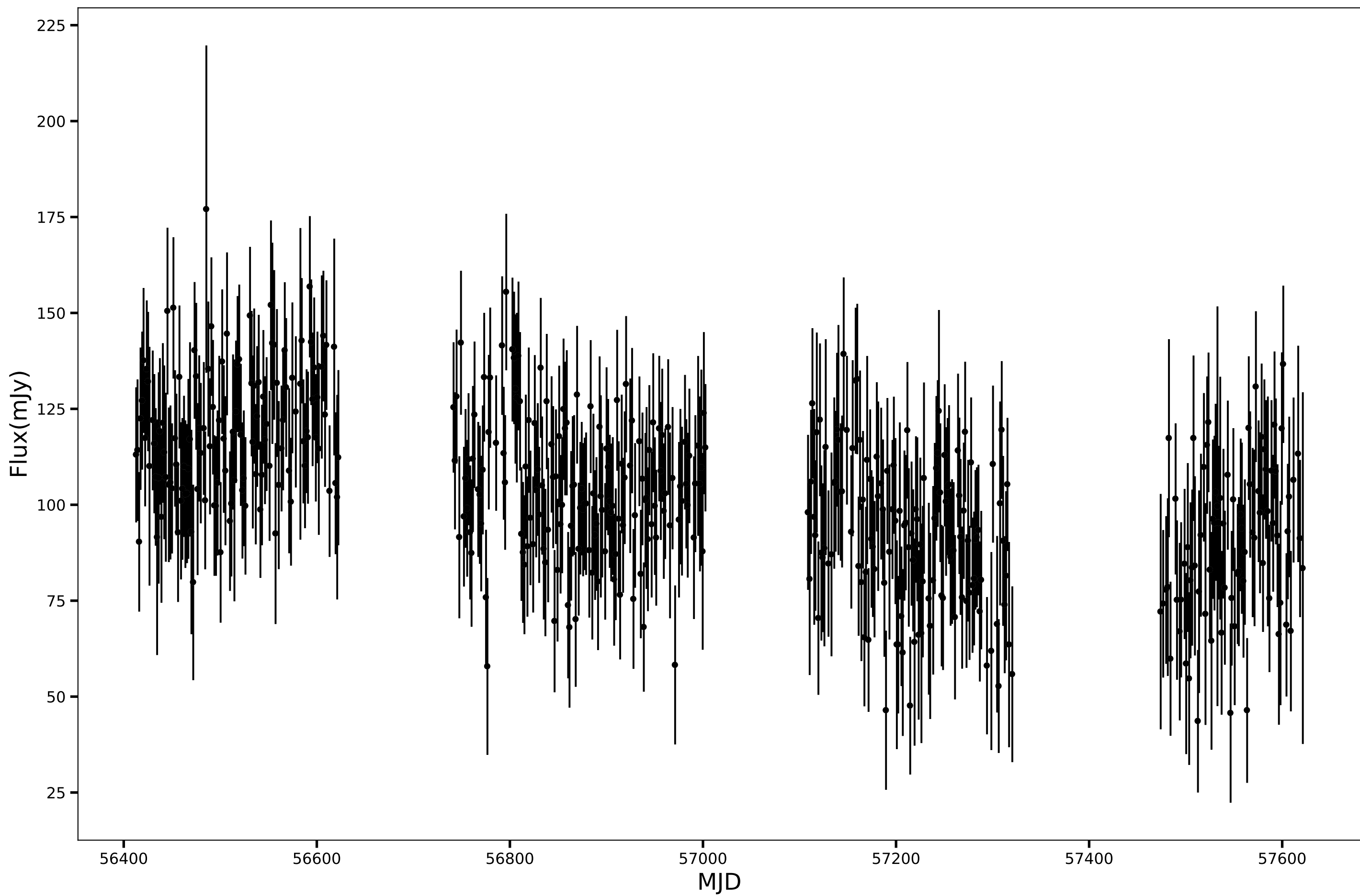
SPT-SJ005856-5219.4, RA=14.7342d, DEC=-52.3244d, mean_flux=102.74 (mJy), 90GHz
