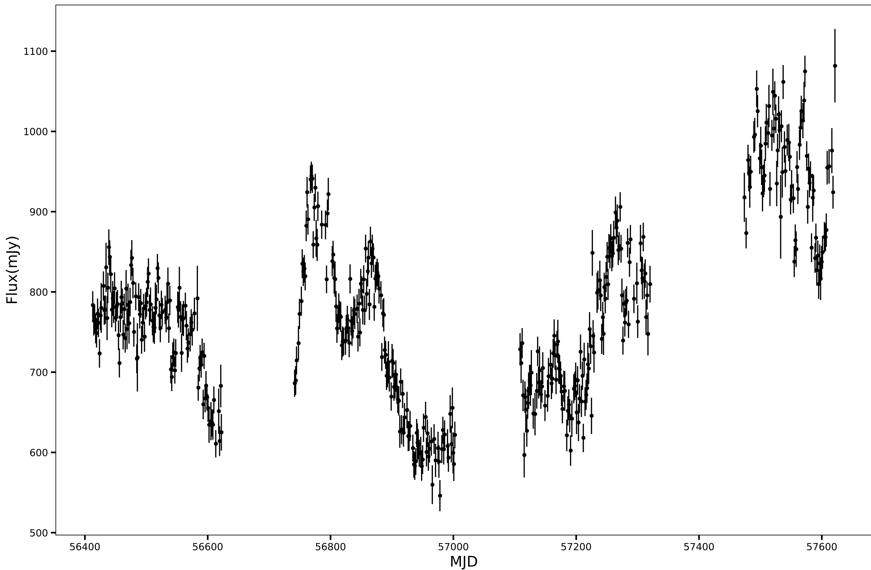
SPT-SJ005846-5659.1, RA=14.6944d, DEC=-56.9855d, mean_flux=777.06 (mJy), 90GHz
