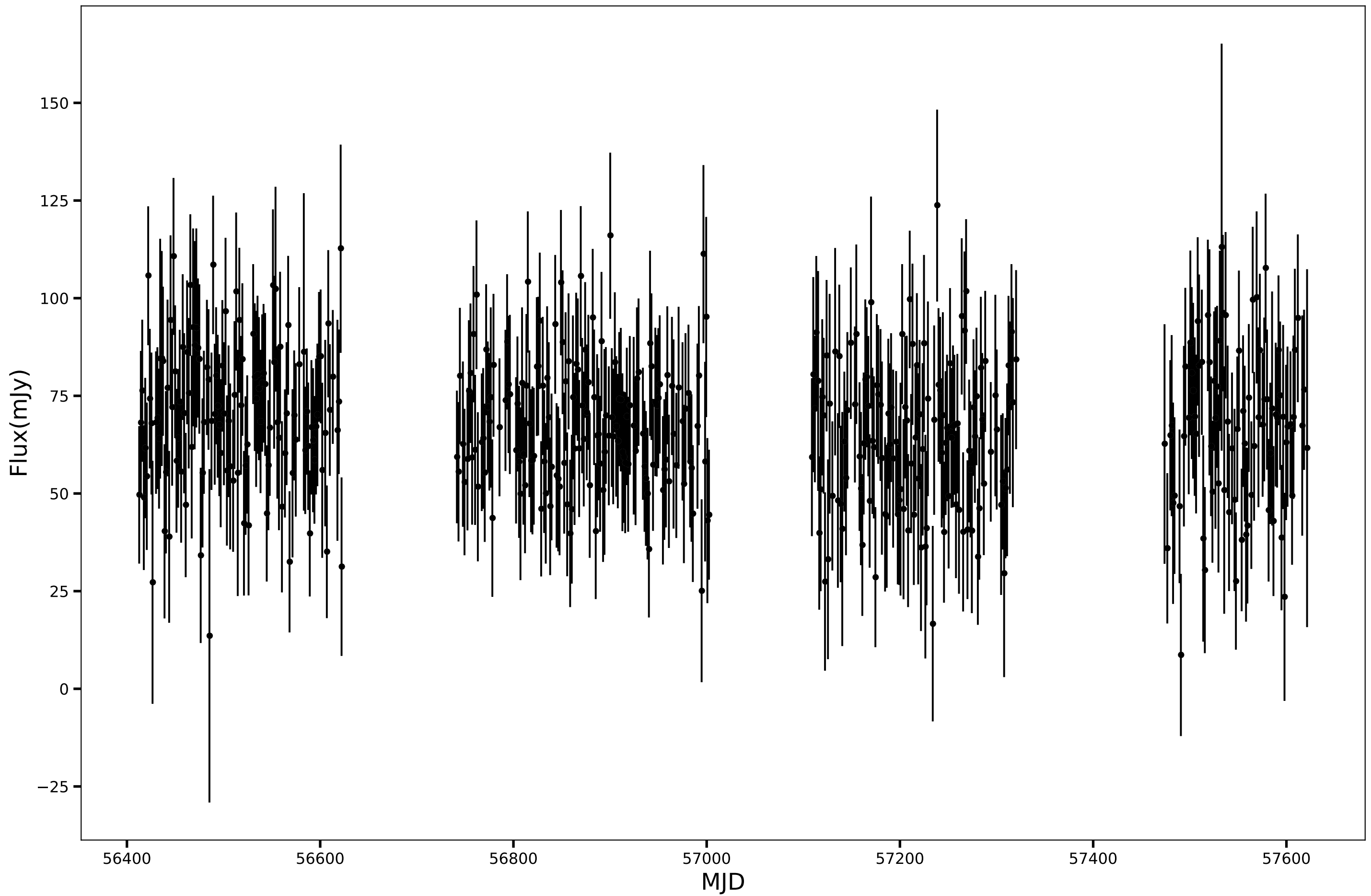
SPT-SJ005705-5214.3, RA=14.2738d, DEC=-52.2392d, mean_flux=67.35 (mJy), 90GHz
