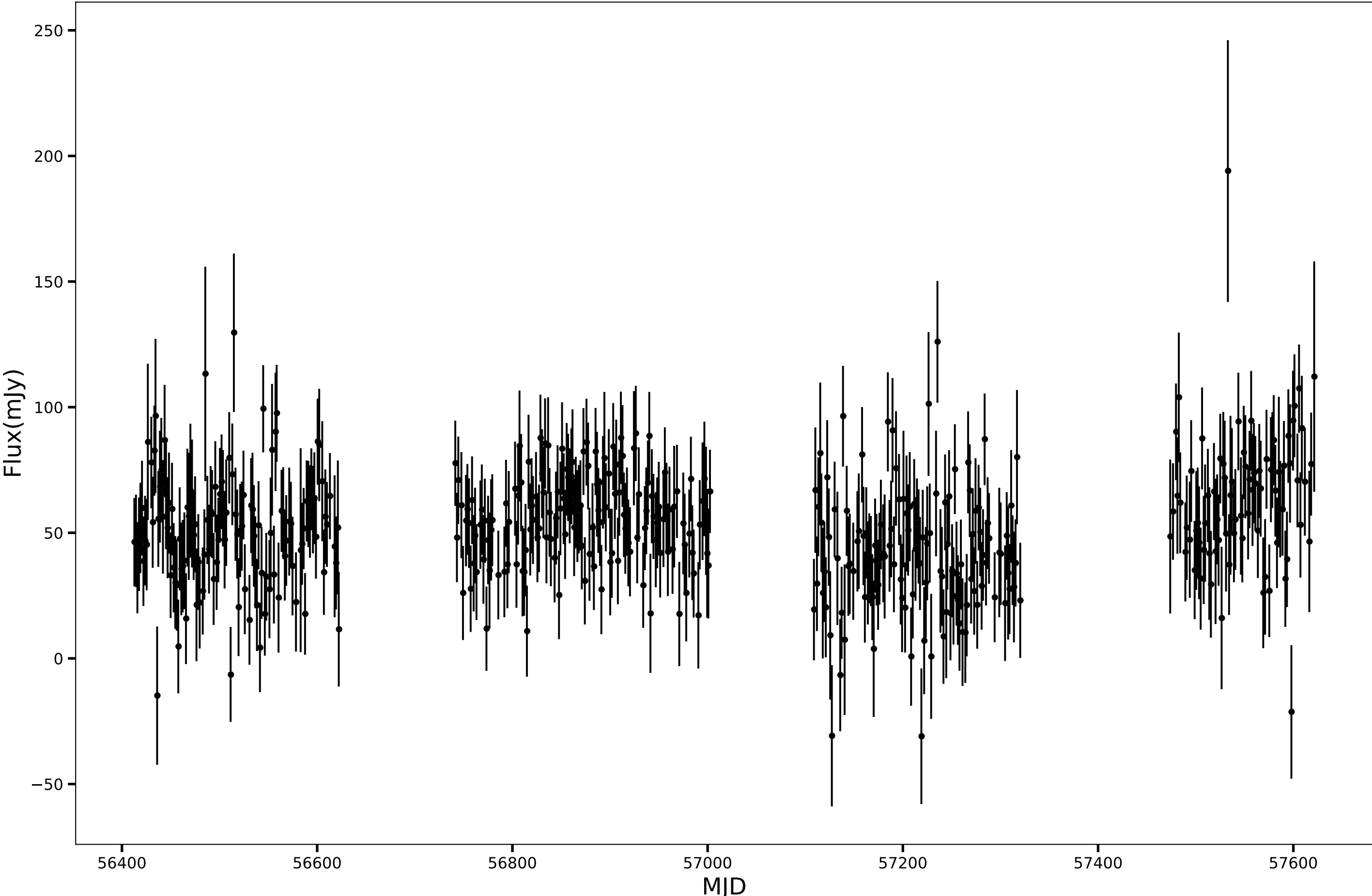
SPT-SJ005243-4947.4, RA=13.1833d, DEC=-49.7910d, mean flux=52.19 (mJy), 90GHz
