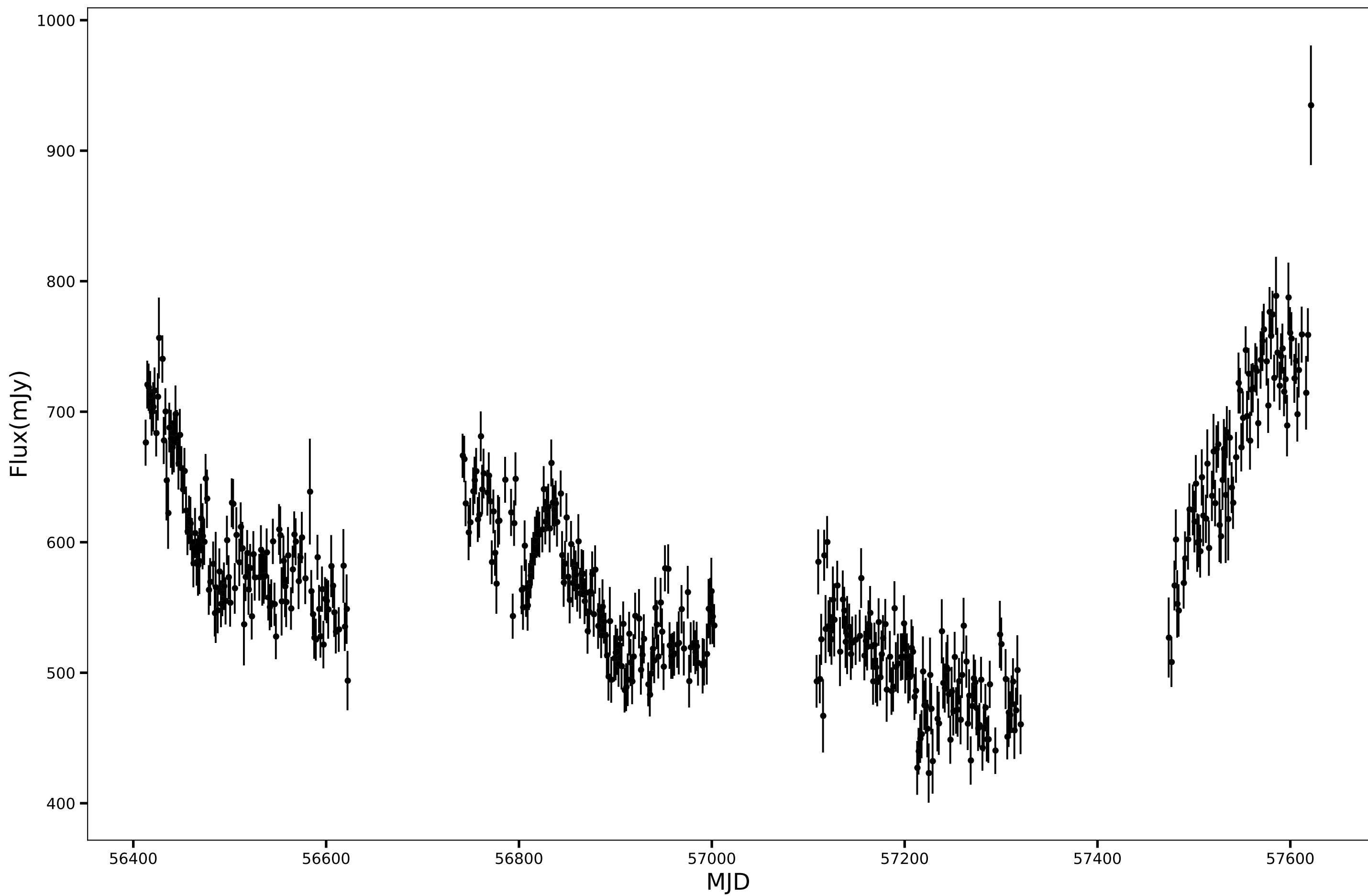
SPT-SJ004959-5738.4, RA=12.4978d, DEC=-57.6400d, mean_flux=576.95 (mJy), 90GHz
