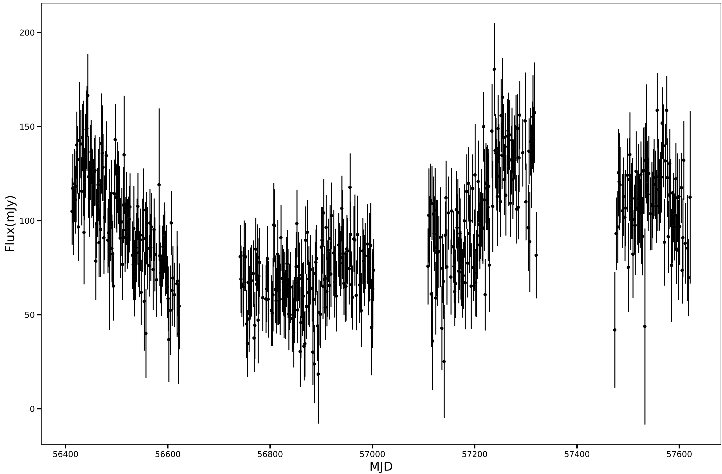
SPT-SJ004905-5521.1, RA=12.2742d, DEC=-55.3524d, mean_flux=93.34 (mJy), 90GHz
