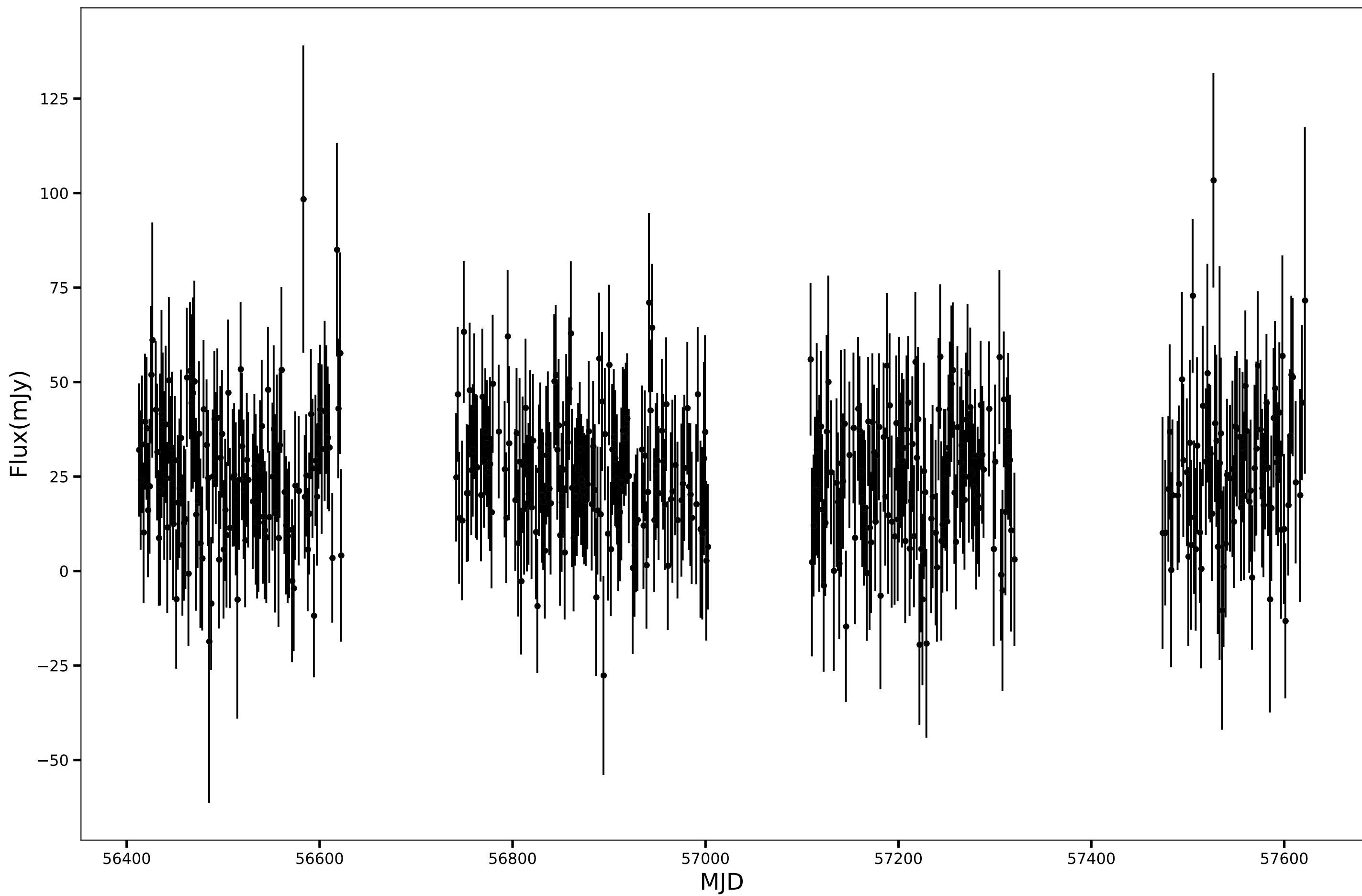
SPT-SJ004520-5447.7, RA=11.3362d, DEC=-54.7951d, mean_flux=25.69 (mJy), 90GHz
